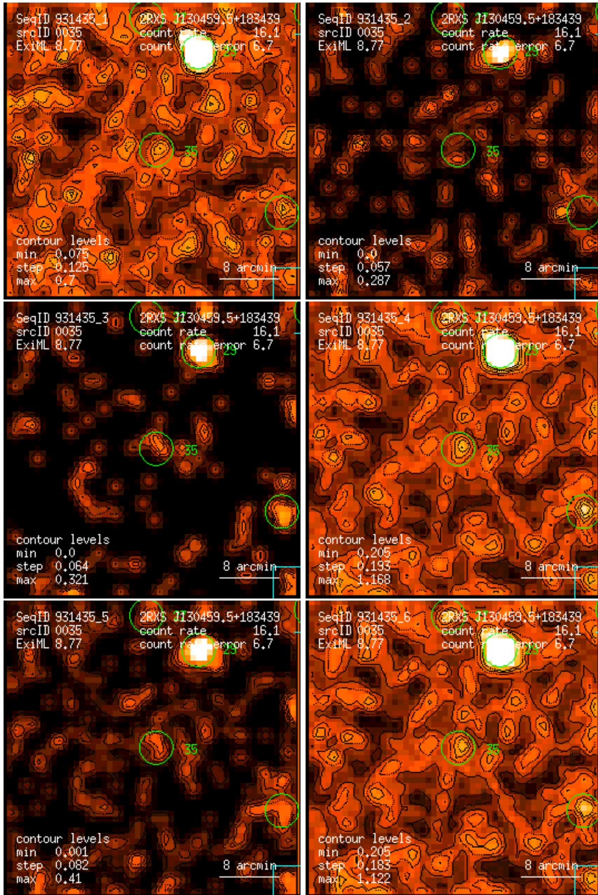
Figure 35: RASS 931435: detection 0035: band rate images, Gaussian filter: (1) PSPC channels 11 – 41, (2) 52 – 90, (3) 91 – 201, (4) 11 – 235, (5) 52 – 201, (6) 11 – 201. Broad band rates in counts/ks. Band rate contour levels in counts/ks/arcmin 2 .
