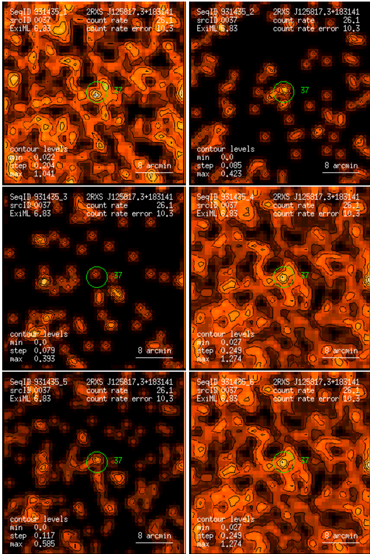
Figure 37: RASS 931435: detection 0037: band rate images, Gaussian filter: (1) PSPC channels 11 – 41, (2) 52 – 90, (3) 91 – 201, (4) 11 – 235, (5) 52 – 201, (6) 11 – 201. Broad band rates in counts/ks. Band rate contour levels in counts/ks/arcmin 2 .
