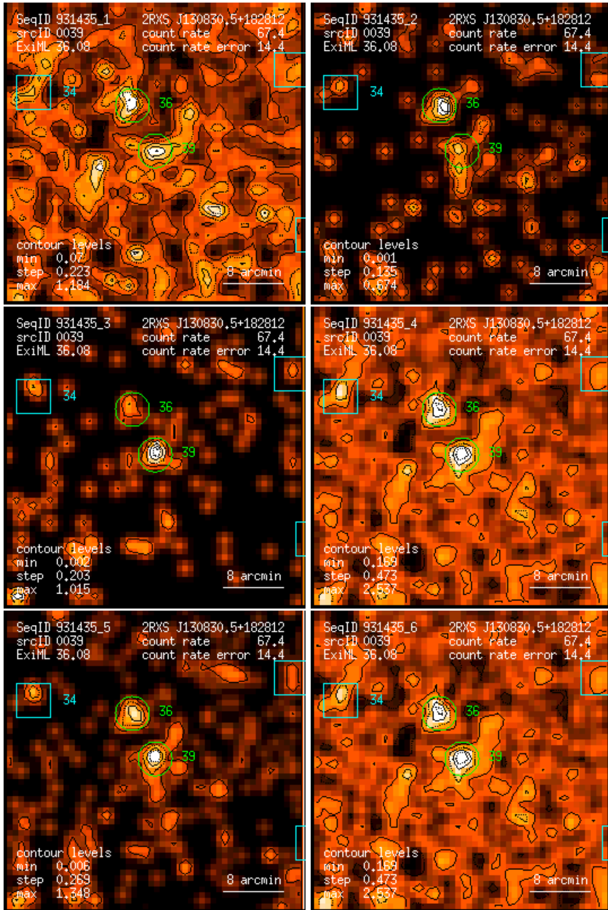
Figure 39: RASS 931435: detection 0039: band rate images, Gaussian filter: (1) PSPC channels 11 – 41, (2) 52 – 90, (3) 91 – 201, (4) 11 – 235, (5) 52 – 201, (6) 11 – 201. Broad band rates in counts/ks. Band rate contour levels in counts/ks/arcmin 2 .
