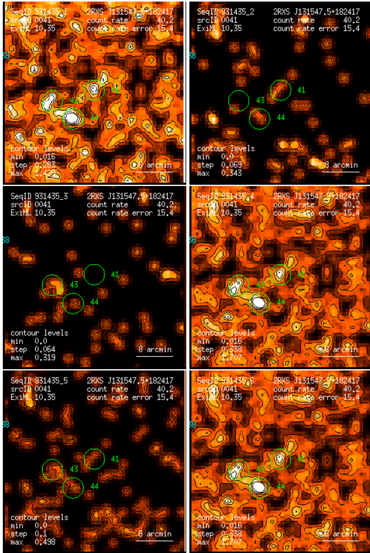
Figure 41: RASS 931435: detection 0041: band rate images, Gaussian filter: (1) PSPC channels 11 – 41, (2) 52 – 90, (3) 91 – 201, (4) 11 – 235, (5) 52 – 201, (6) 11 – 201. Broad band rates in counts/ks. Band rate contour levels in counts/ks/arcmin 2 .
