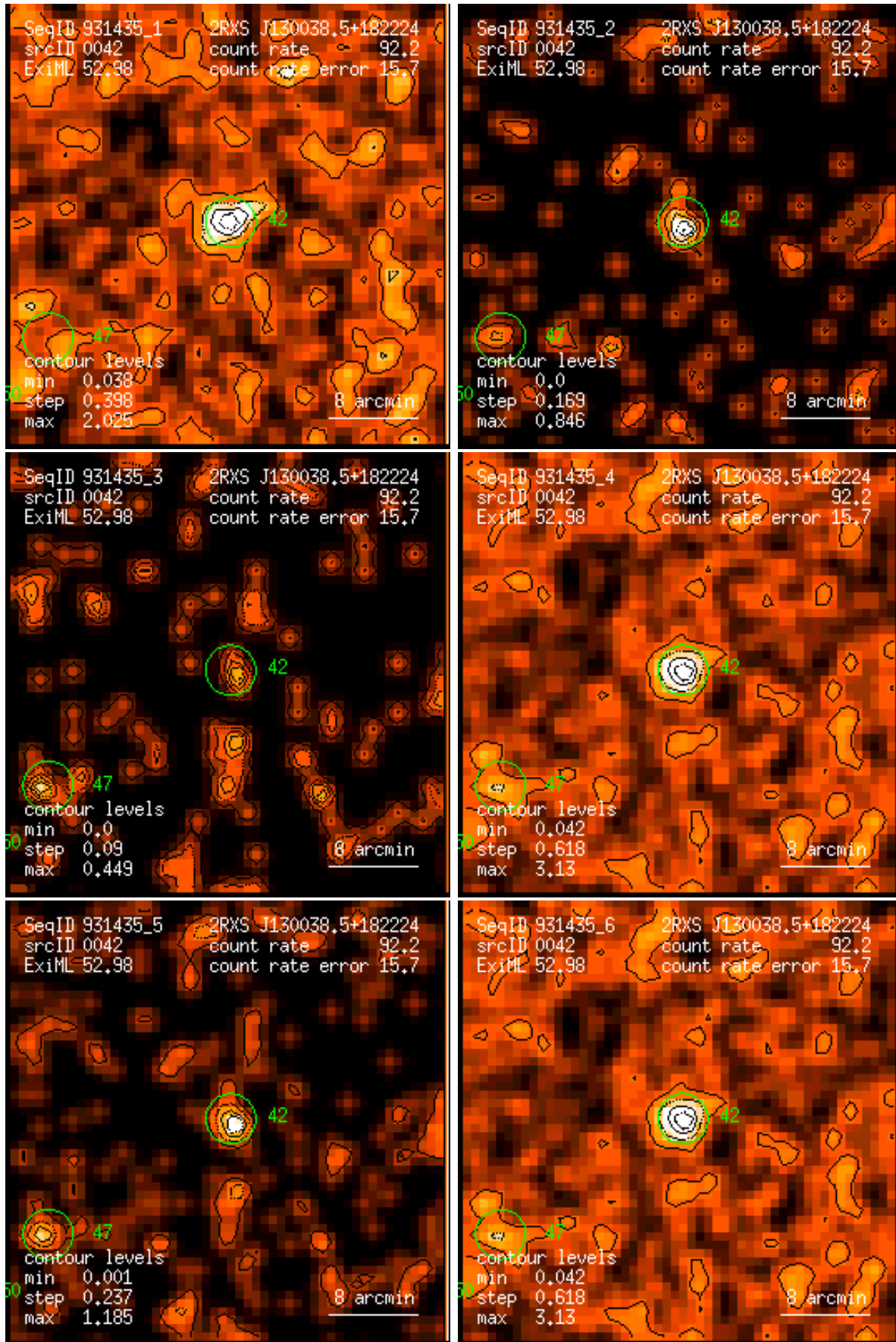
Figure 42: RASS 931435: detection 0042: band rate images, Gaussian filter: (1) PSPC channels 11 – 41, (2) 52 – 90, (3) 91 – 201, (4) 11 – 235, (5) 52 – 201, (6) 11 – 201. Broad band rates in counts/ks. Band rate contour levels in counts/ks/arcmin 2 .
