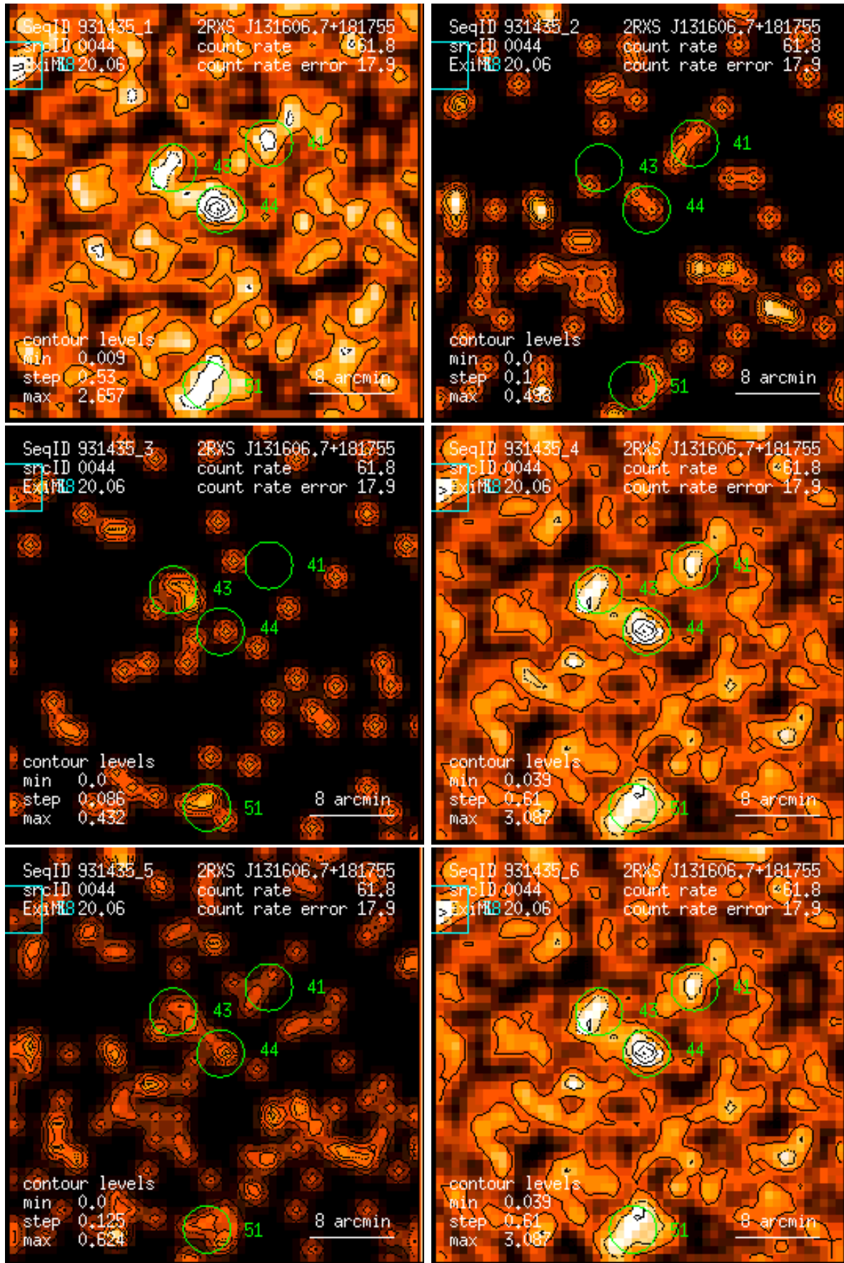
Figure 44: RASS 931435: detection 0044: band rate images, Gaussian filter: (1) PSPC channels 11 – 41, (2) 52 – 90, (3) 91 – 201, (4) 11 – 235, (5) 52 – 201, (6) 11 – 201. Broad band rates in counts/ks. Band rate contour levels in counts/ks/arcmin 2 .
