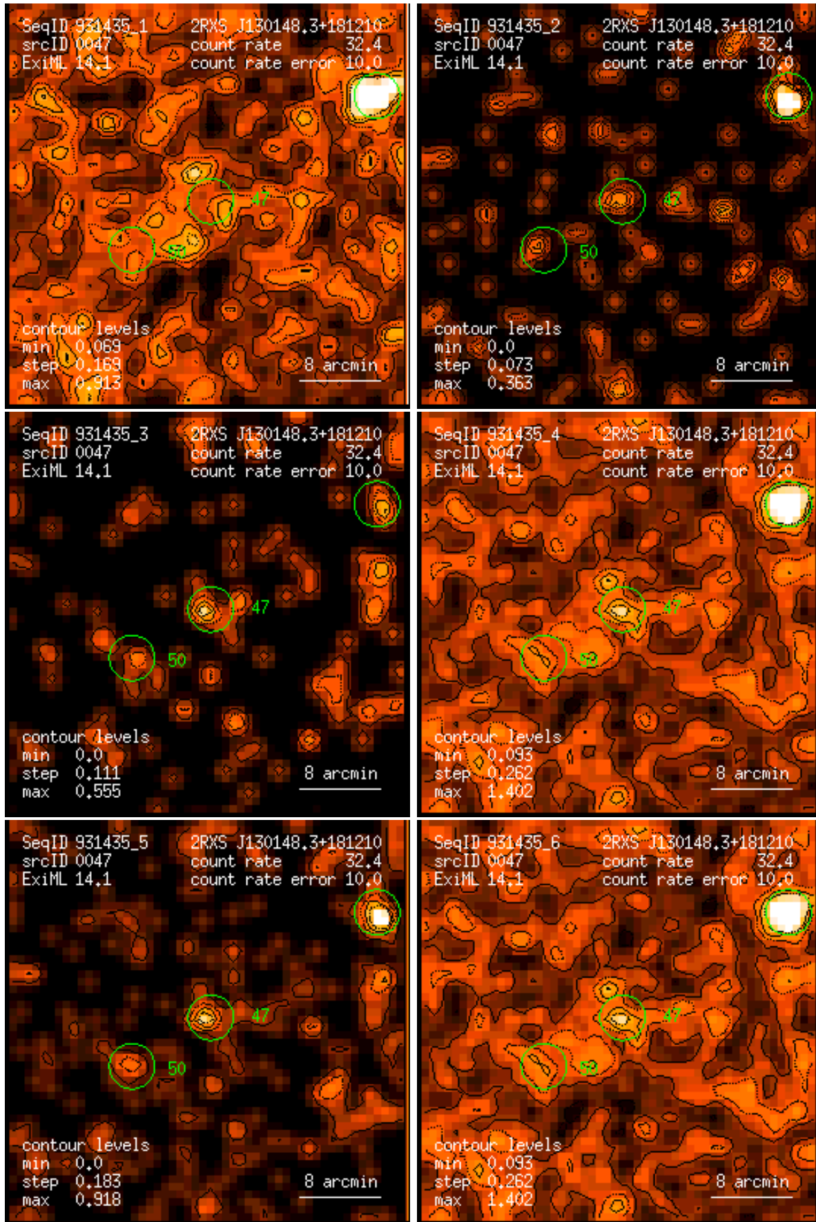
Figure 47: RASS 931435: detection 0047: band rate images, Gaussian filter: (1) PSPC channels 11 – 41, (2) 52 – 90, (3) 91 – 201, (4) 11 – 235, (5) 52 – 201, (6) 11 – 201. Broad band rates in counts/ks. Band rate contour levels in counts/ks/arcmin 2 .
