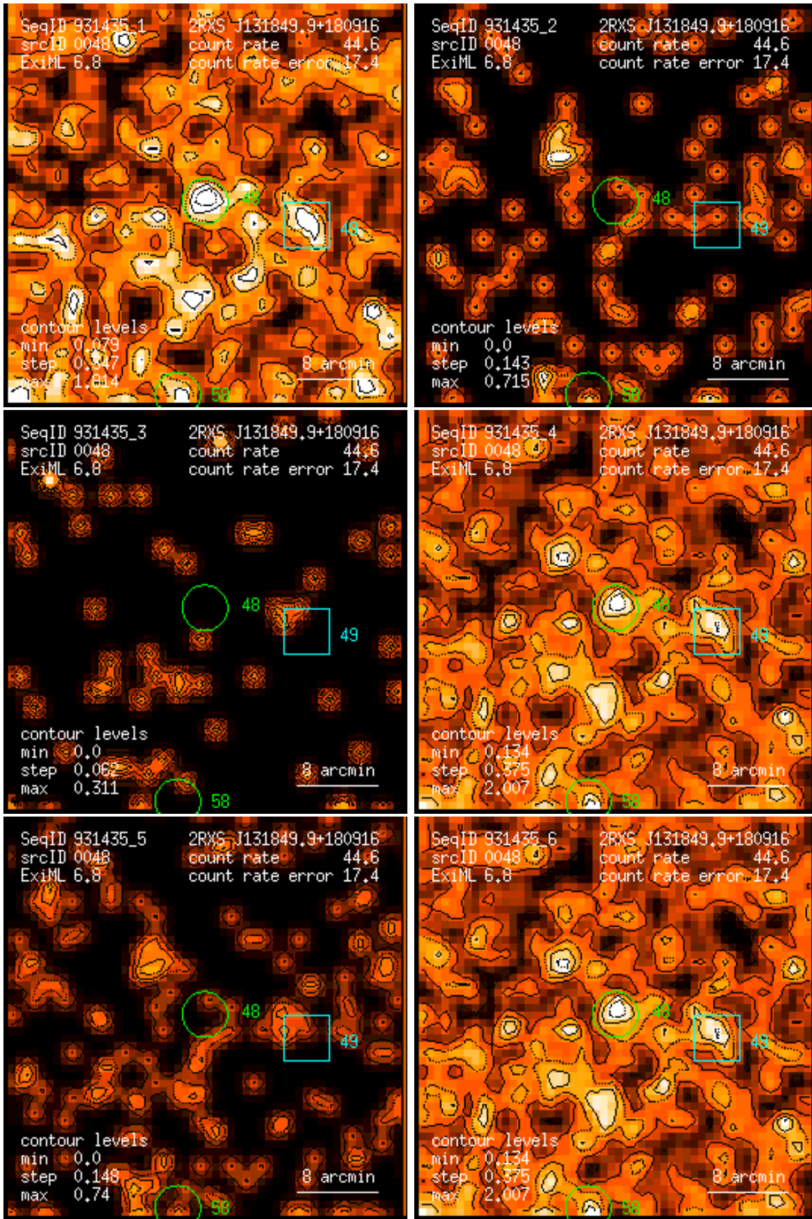
Figure 48: RASS 931435: detection 0048: band rate images, Gaussian filter: (1) PSPC channels 11 – 41, (2) 52 – 90, (3) 91 – 201, (4) 11 – 235, (5) 52 – 201, (6) 11 – 201. Broad band rates in counts/ks. Band rate contour levels in counts/ks/arcmin 2 .
