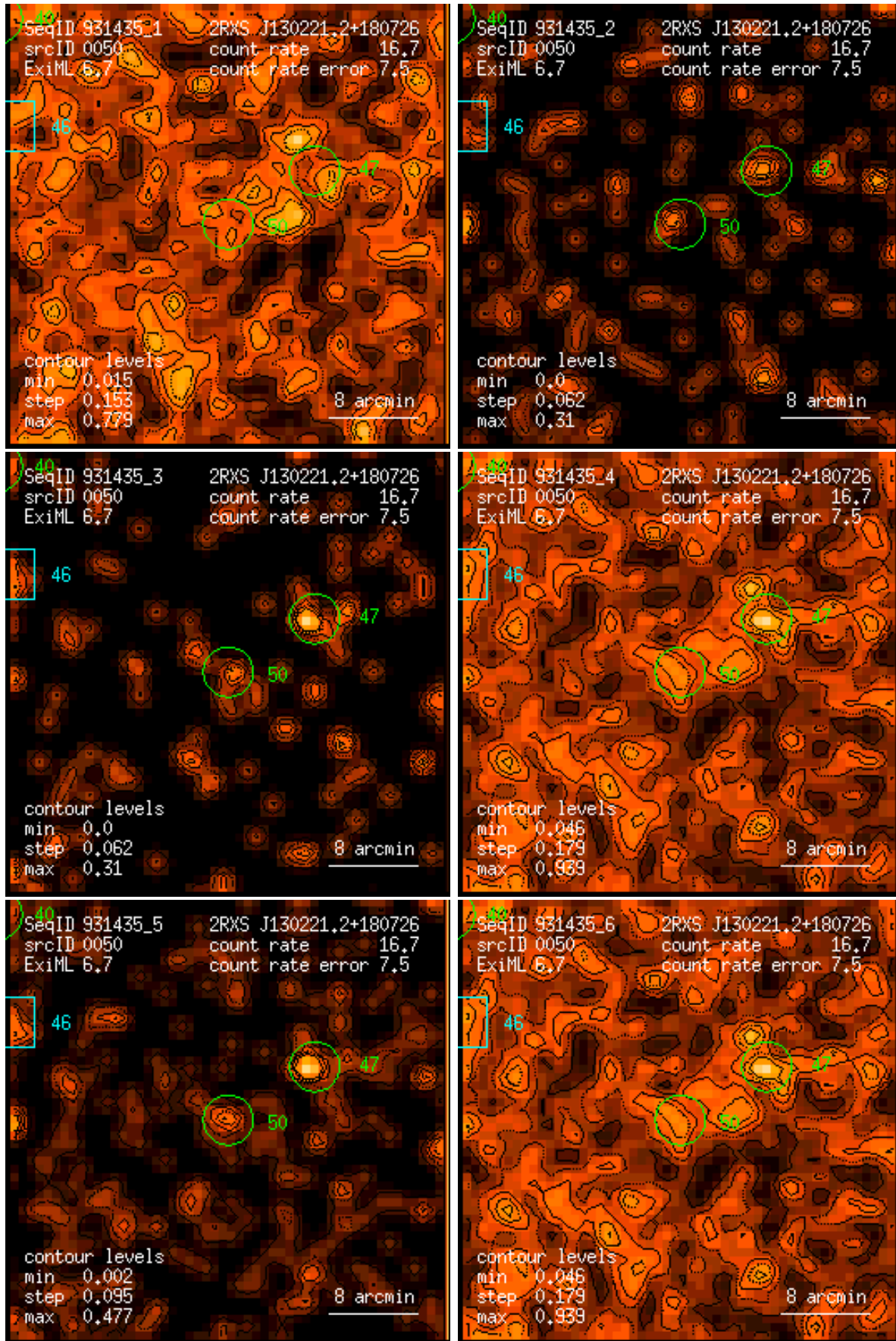
Figure 50: RASS 931435: detection 0050: band rate images, Gaussian filter: (1) PSPC channels 11 – 41, (2) 52 – 90, (3) 91 – 201, (4) 11 – 235, (5) 52 – 201, (6) 11 – 201. Broad band rates in counts/ks. Band rate contour levels in counts/ks/arcmin 2 .
