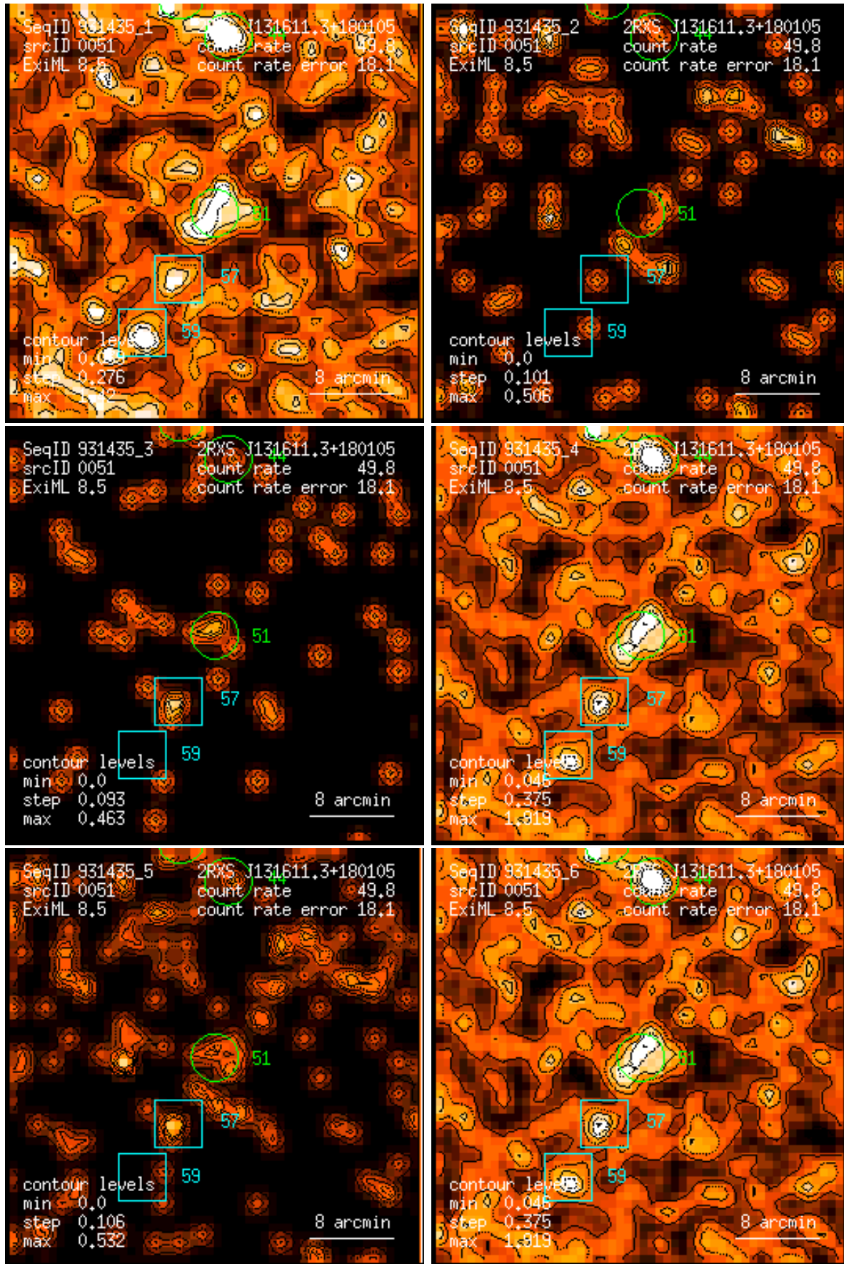
Figure 51: RASS 931435: detection 0051: band rate images, Gaussian filter: (1) PSPC channels 11 – 41, (2) 52 – 90, (3) 91 – 201, (4) 11 – 235, (5) 52 – 201, (6) 11 – 201. Broad band rates in counts/ks. Band rate contour levels in counts/ks/arcmin 2 .
