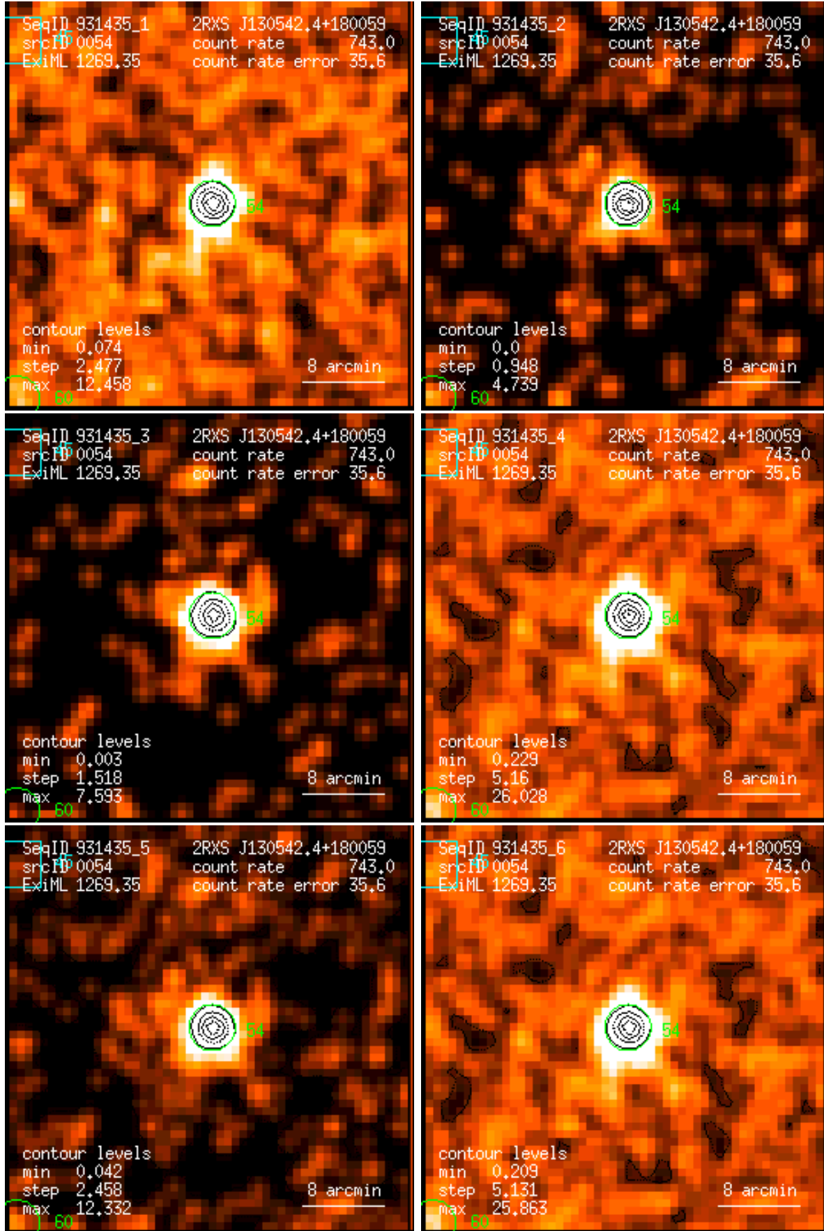
Figure 54: RASS 931435: detection 0054: band rate images, Gaussian filter: (1) PSPC channels 11 – 41, (2) 52 – 90, (3) 91 – 201, (4) 11 – 235, (5) 52 – 201, (6) 11 – 201. Broad band rates in counts/ks. Band rate contour levels in counts/ks/arcmin 2 .
