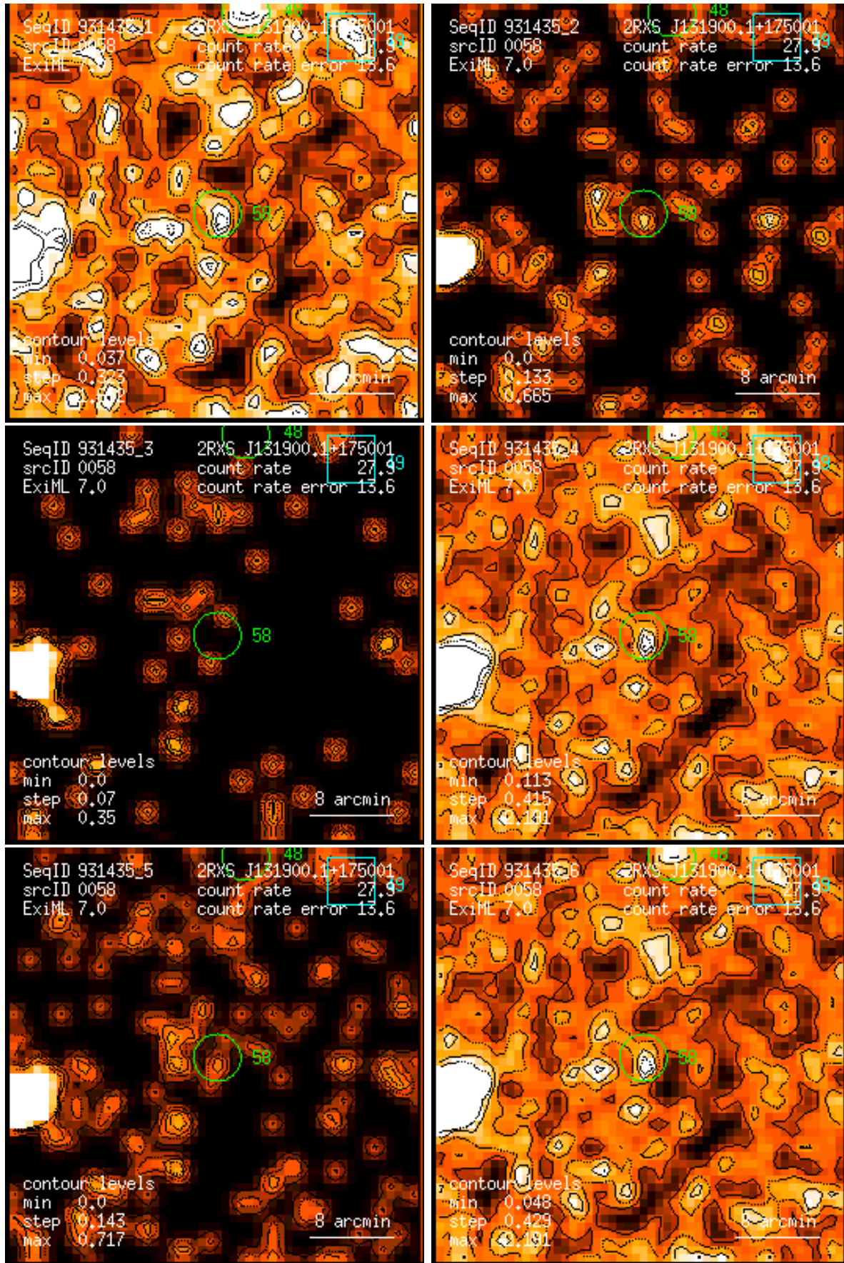
Figure 58: RASS 931435: detection 0058: band rate images, Gaussian filter: (1) PSPC channels 11 – 41, (2) 52 – 90, (3) 91 – 201, (4) 11 – 235, (5) 52 – 201, (6) 11 – 201. Broad band rates in counts/ks. Band rate contour levels in counts/ks/arcmin 2 .
