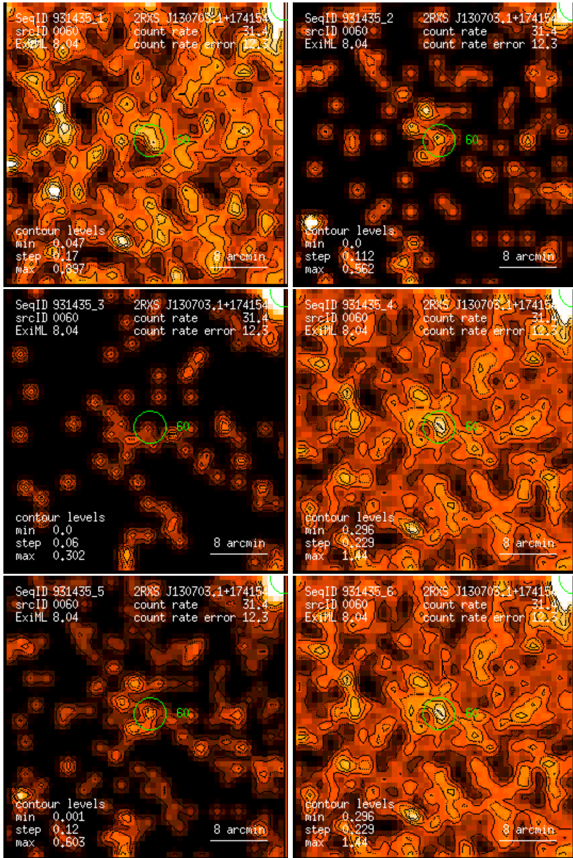
Figure 60: RASS 931435: detection 0060: band rate images, Gaussian filter: (1) PSPC channels 11 – 41, (2) 52 – 90, (3) 91 – 201, (4) 11 – 235, (5) 52 – 201, (6) 11 – 201. Broad band rates in counts/ks. Band rate contour levels in counts/ks/arcmin 2 .
