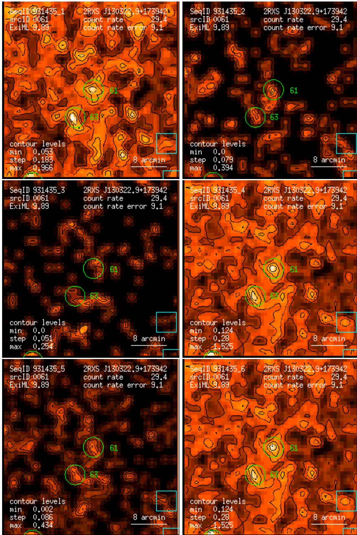
Figure 61: RASS 931435: detection 0061: band rate images, Gaussian filter: (1) PSPC channels 11 – 41, (2) 52 – 90, (3) 91 – 201, (4) 11 – 235, (5) 52 – 201, (6) 11 – 201. Broad band rates in counts/ks. Band rate contour levels in counts/ks/arcmin 2 .
