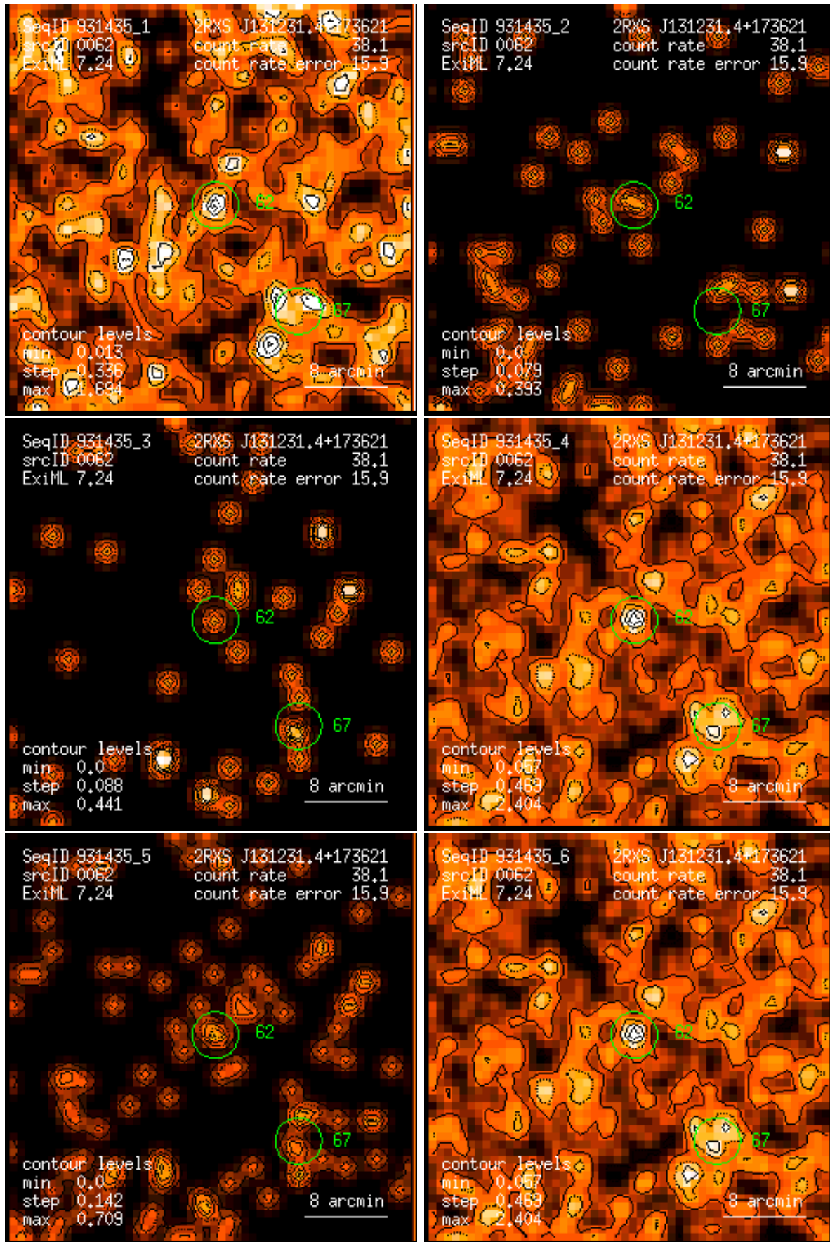
Figure 62: RASS 931435: detection 0062: band rate images, Gaussian filter: (1) PSPC channels 11 – 41, (2) 52 – 90, (3) 91 – 201, (4) 11 – 235, (5) 52 – 201, (6) 11 – 201. Broad band rates in counts/ks. Band rate contour levels in counts/ks/arcmin 2 .
