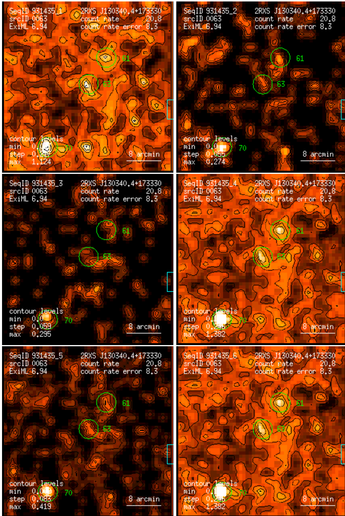
Figure 63: RASS 931435: detection 0063: band rate images, Gaussian filter: (1) PSPC channels 11 – 41, (2) 52 – 90, (3) 91 – 201, (4) 11 – 235, (5) 52 – 201, (6) 11 – 201. Broad band rates in counts/ks. Band rate contour levels in counts/ks/arcmin 2 .
