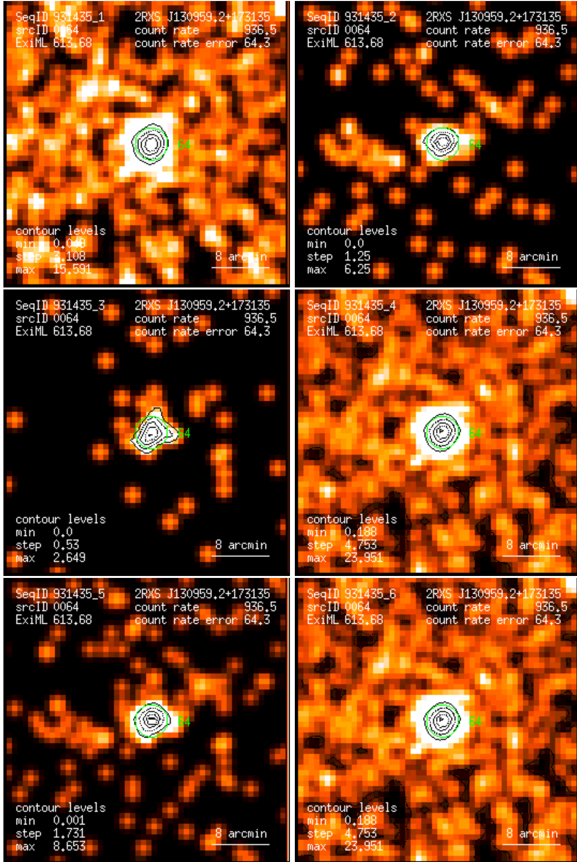
Figure 64: RASS 931435: detection 0064: band rate images, Gaussian filter: (1) PSPC channels 11 – 41, (2) 52 – 90, (3) 91 – 201, (4) 11 – 235, (5) 52 – 201, (6) 11 – 201. Broad band rates in counts/ks. Band rate contour levels in counts/ks/arcmin 2 .
