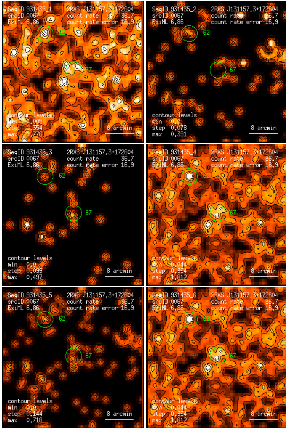
Figure 67: RASS 931435: detection 0067: band rate images, Gaussian filter: (1) PSPC channels 11 – 41, (2) 52 – 90, (3) 91 – 201, (4) 11 – 235, (5) 52 – 201, (6) 11 – 201. Broad band rates in counts/ks. Band rate contour levels in counts/ks/arcmin 2 .
