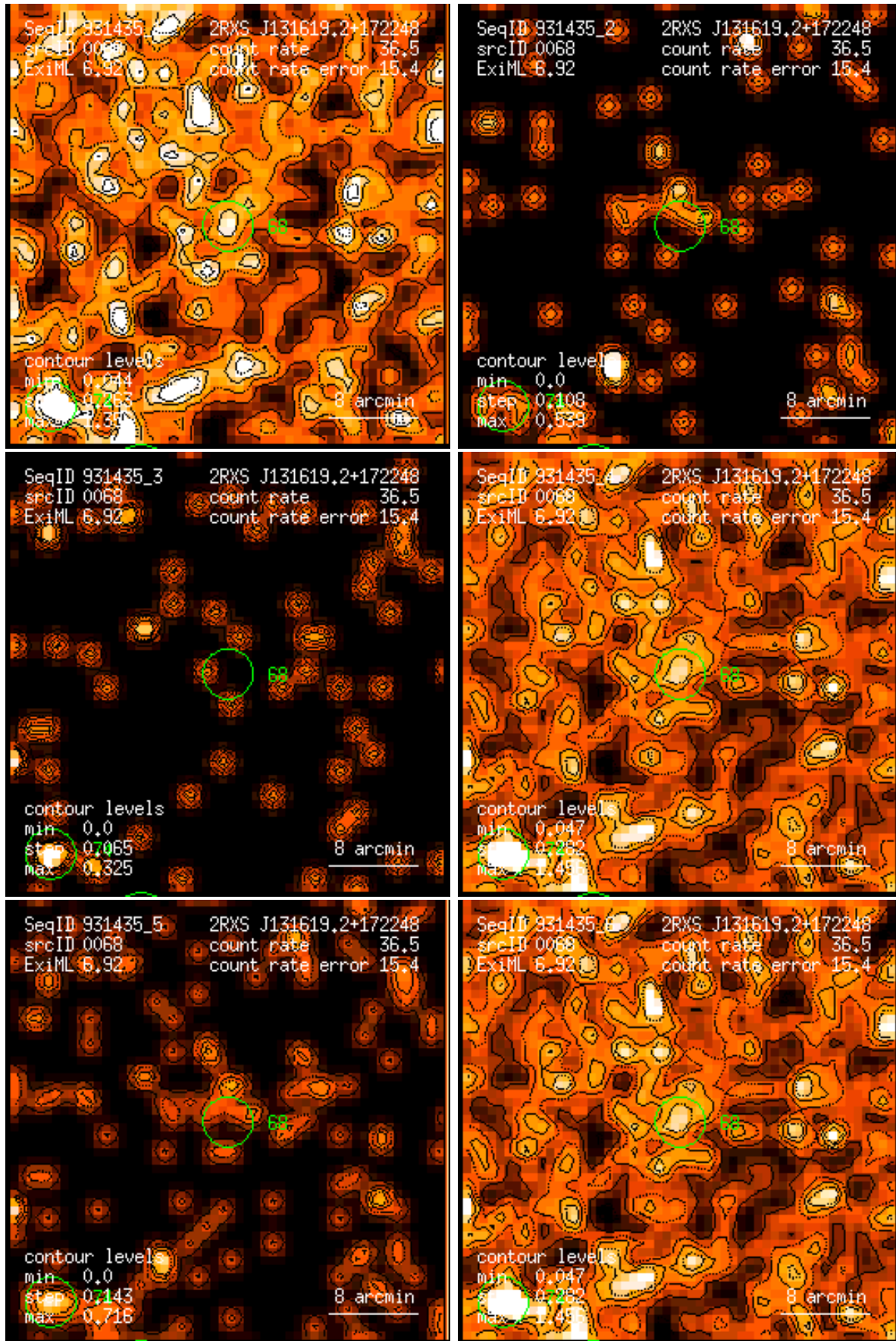
Figure 68: RASS 931435: detection 0068: band rate images, Gaussian filter: (1) PSPC channels 11 – 41, (2) 52 – 90, (3) 91 – 201, (4) 11 – 235, (5) 52 – 201, (6) 11 – 201. Broad band rates in counts/ks. Band rate contour levels in counts/ks/arcmin 2 .
