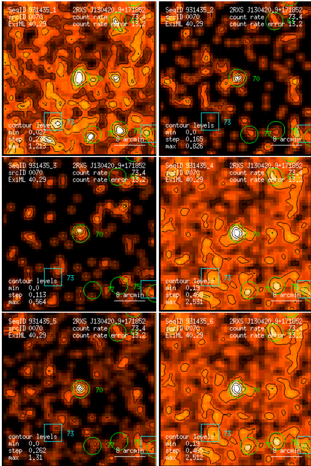
Figure 70: RASS 931435: detection 0070: band rate images, Gaussian filter: (1) PSPC channels 11 – 41, (2) 52 – 90, (3) 91 – 201, (4) 11 – 235, (5) 52 – 201, (6) 11 – 201. Broad band rates in counts/ks. Band rate contour levels in counts/ks/arcmin 2 .
