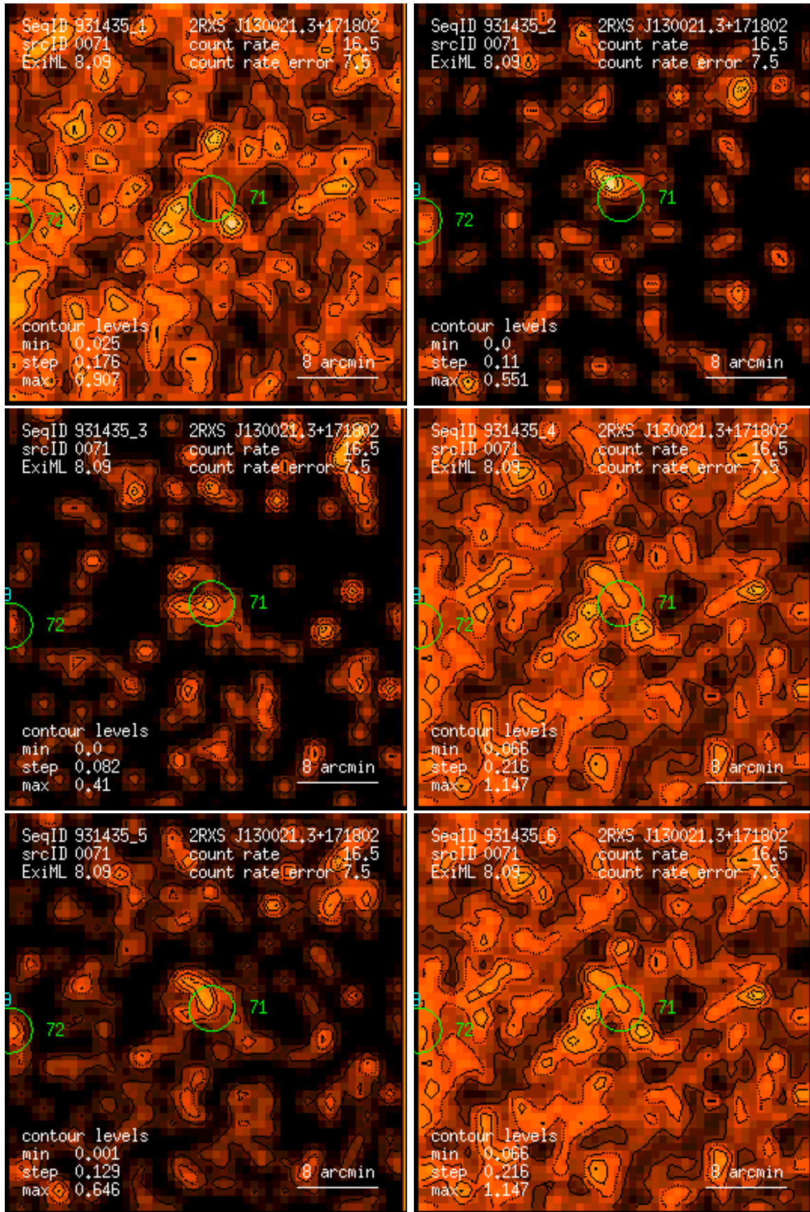
Figure 71: RASS 931435: detection 0071: band rate images, Gaussian filter: (1) PSPC channels 11 – 41, (2) 52 – 90, (3) 91 – 201, (4) 11 – 235, (5) 52 – 201, (6) 11 – 201. Broad band rates in counts/ks. Band rate contour levels in counts/ks/arcmin 2 .
