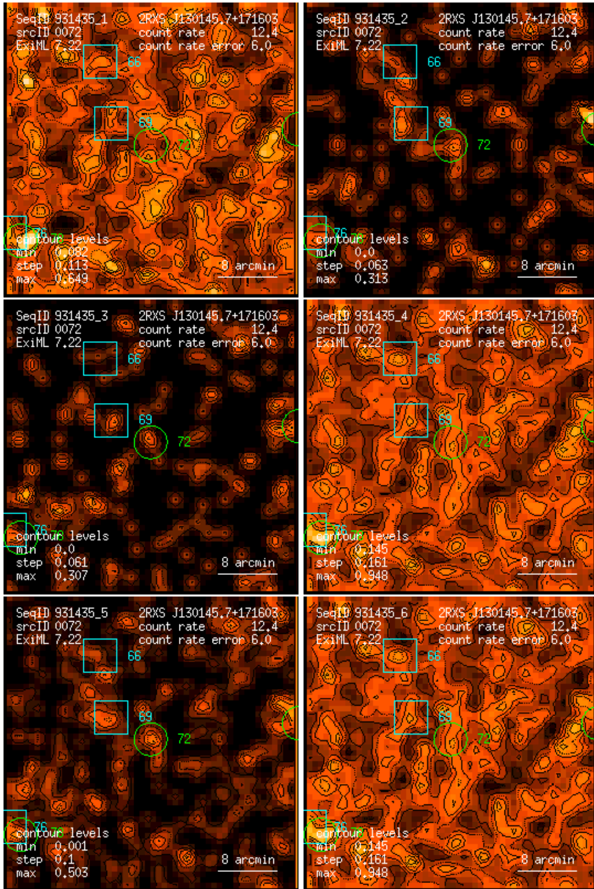
Figure 72: RASS 931435: detection 0072: band rate images, Gaussian filter: (1) PSPC channels 11 – 41, (2) 52 – 90, (3) 91 – 201, (4) 11 – 235, (5) 52 – 201, (6) 11 – 201. Broad band rates in counts/ks. Band rate contour levels in counts/ks/arcmin 2 .
