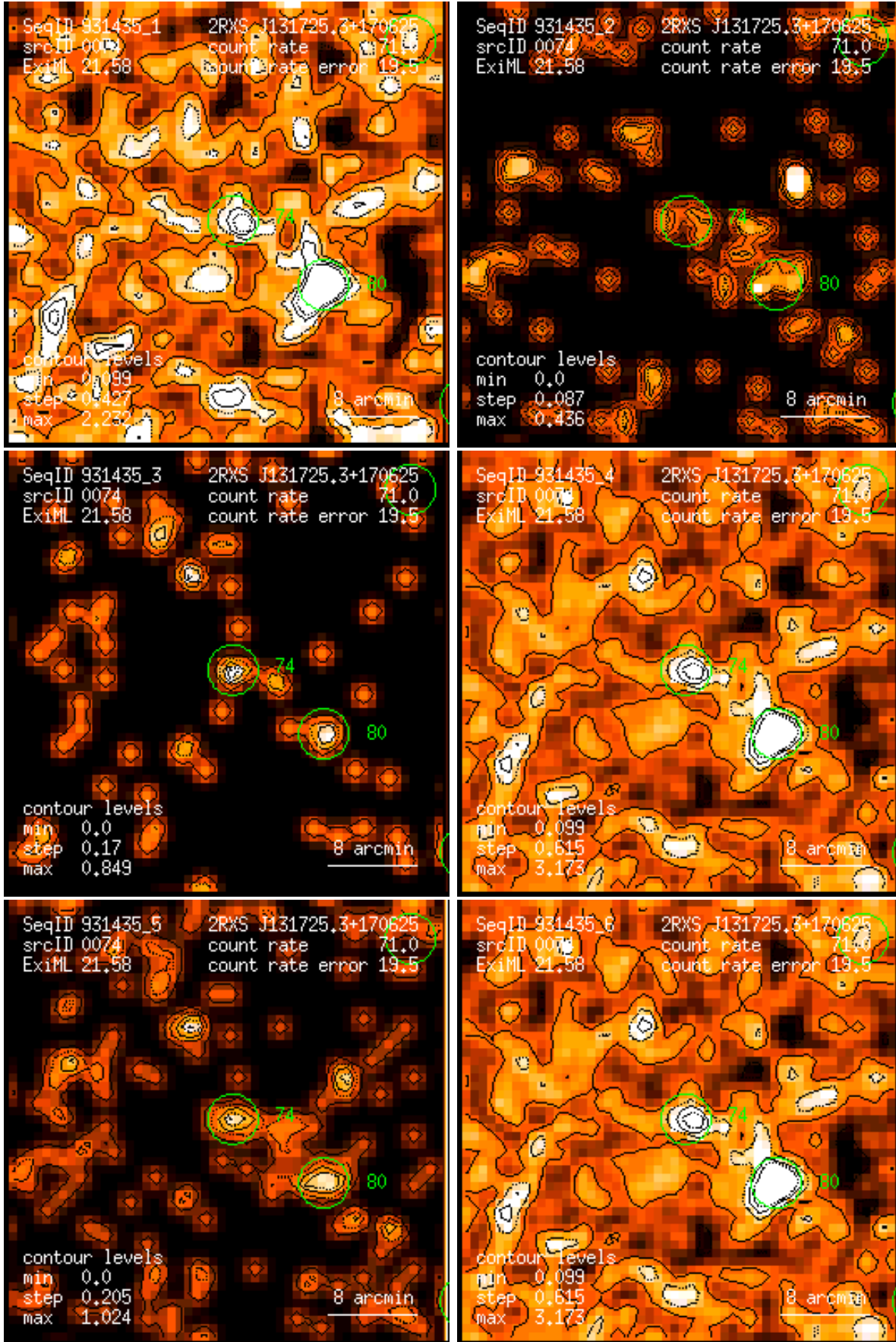
Figure 74: RASS 931435: detection 0074: band rate images, Gaussian filter: (1) PSPC channels 11 – 41, (2) 52 – 90, (3) 91 – 201, (4) 11 – 235, (5) 52 – 201, (6) 11 – 201. Broad band rates in counts/ks. Band rate contour levels in counts/ks/arcmin 2 .
