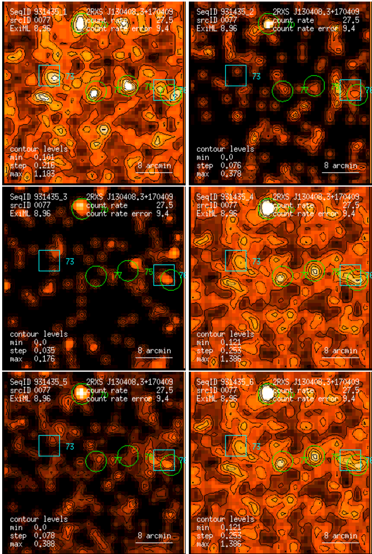
Figure 77: RASS 931435: detection 0077: band rate images, Gaussian filter: (1) PSPC channels 11 – 41, (2) 52 – 90, (3) 91 – 201, (4) 11 – 235, (5) 52 – 201, (6) 11 – 201. Broad band rates in counts/ks. Band rate contour levels in counts/ks/arcmin 2 .
