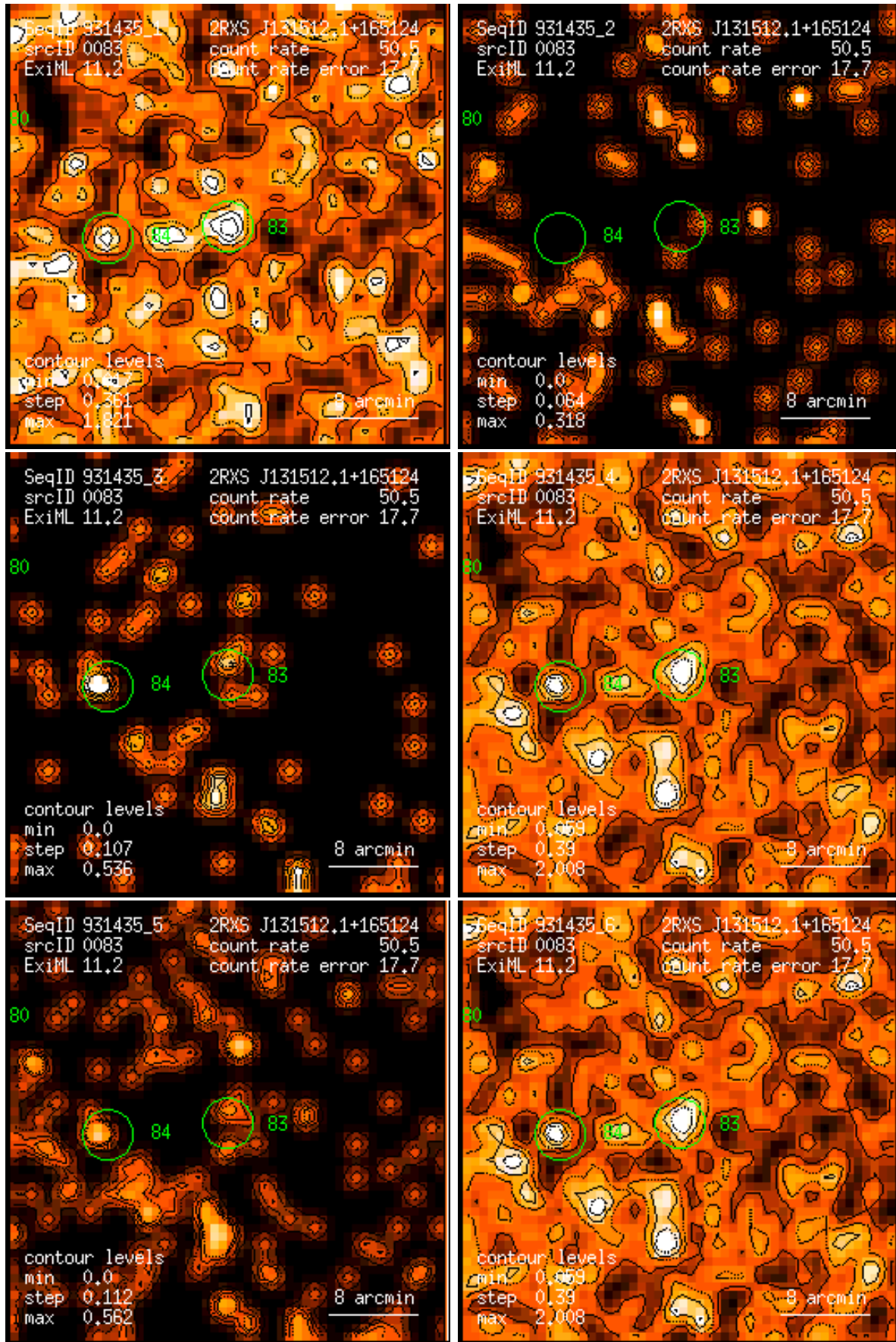
Figure 83: RASS 931435: detection 0083: band rate images, Gaussian filter: (1) PSPC channels 11 – 41, (2) 52 – 90, (3) 91 – 201, (4) 11 – 235, (5) 52 – 201, (6) 11 – 201. Broad band rates in counts/ks. Band rate contour levels in counts/ks/arcmin 2 .
