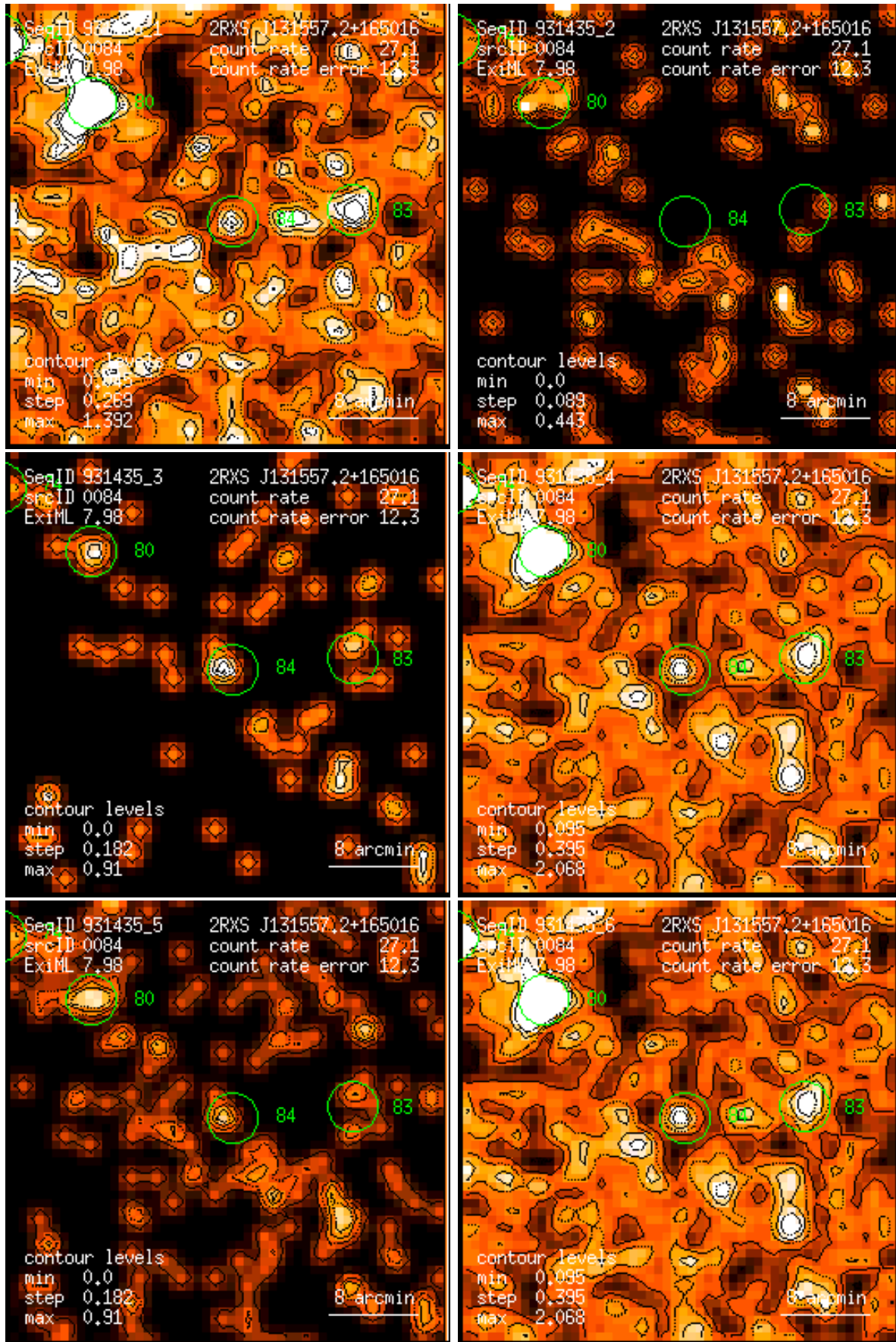
Figure 84: RASS 931435: detection 0084: band rate images, Gaussian filter: (1) PSPC channels 11 – 41, (2) 52 – 90, (3) 91 – 201, (4) 11 – 235, (5) 52 – 201, (6) 11 – 201. Broad band rates in counts/ks. Band rate contour levels in counts/ks/arcmin 2 .
