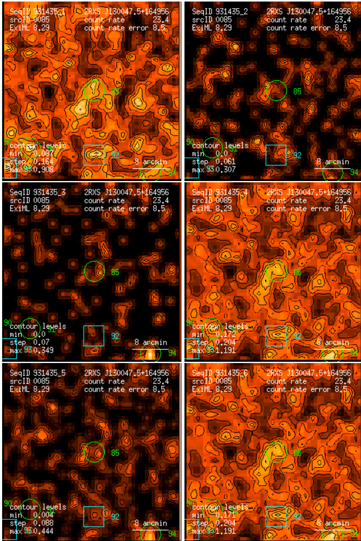
Figure 85: RASS 931435: detection 0085: band rate images, Gaussian filter: (1) PSPC channels 11 – 41, (2) 52 – 90, (3) 91 – 201, (4) 11 – 235, (5) 52 – 201, (6) 11 – 201. Broad band rates in counts/ks. Band rate contour levels in counts/ks/arcmin 2 .
