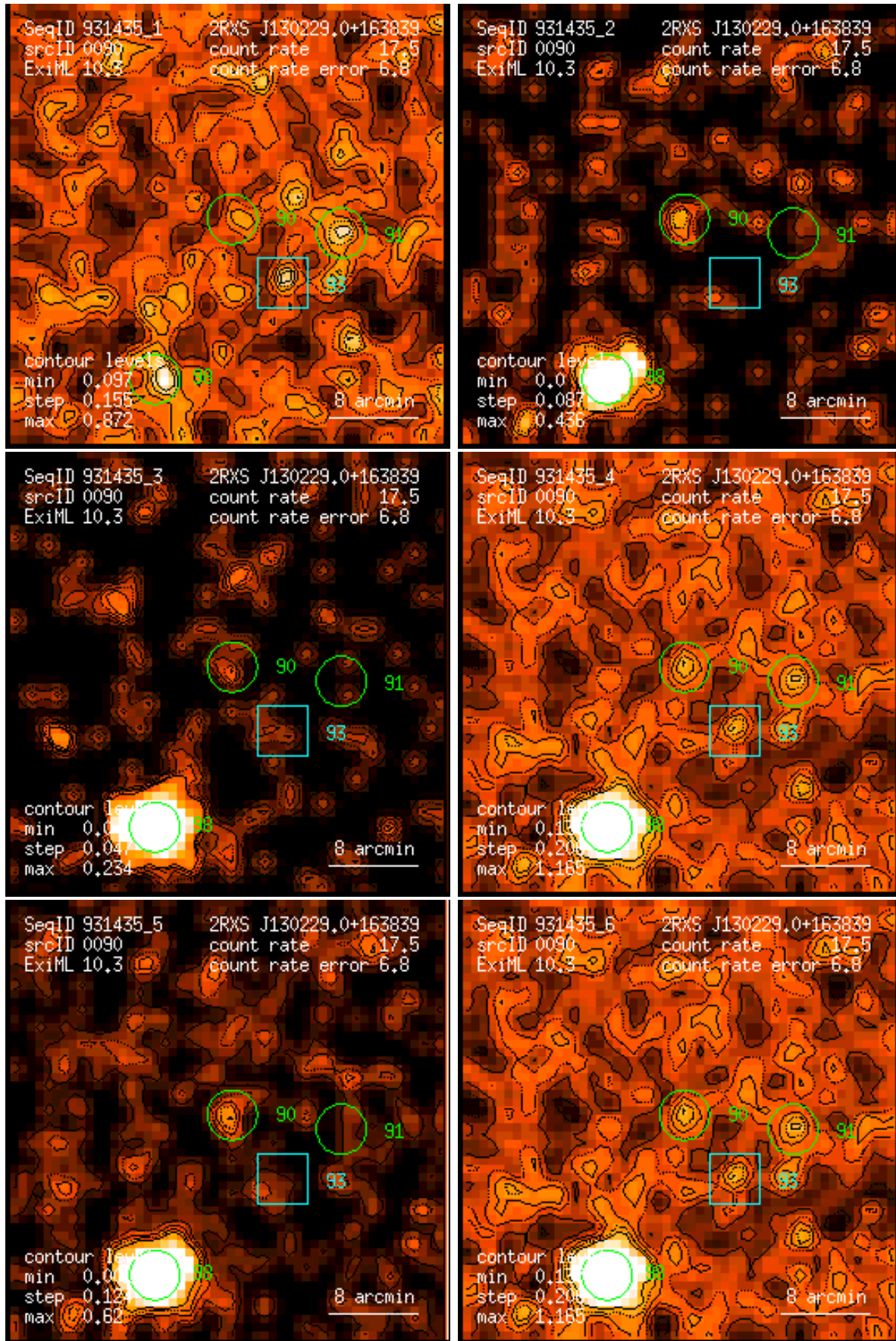
Figure 90: RASS 931435: detection 0090: band rate images, Gaussian filter: (1) PSPC channels 11 – 41, (2) 52 – 90, (3) 91 – 201, (4) 11 – 235, (5) 52 – 201, (6) 11 – 201. Broad band rates in counts/ks. Band rate contour levels in counts/ks/arcmin 2 .
