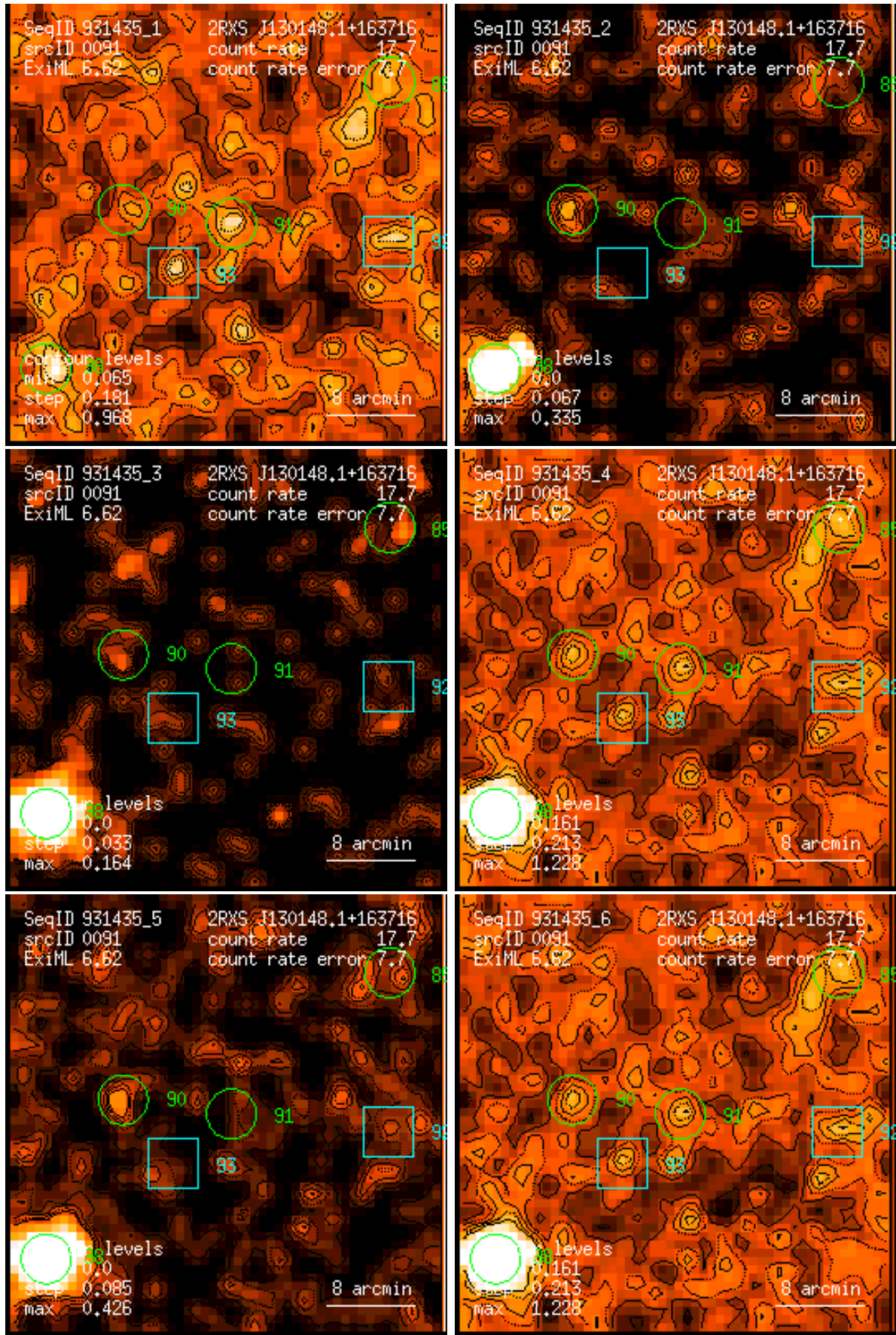
Figure 91: RASS 931435: detection 0091: band rate images, Gaussian filter: (1) PSPC channels 11 – 41, (2) 52 – 90, (3) 91 – 201, (4) 11 – 235, (5) 52 – 201, (6) 11 – 201. Broad band rates in counts/ks. Band rate contour levels in counts/ks/arcmin 2 .
