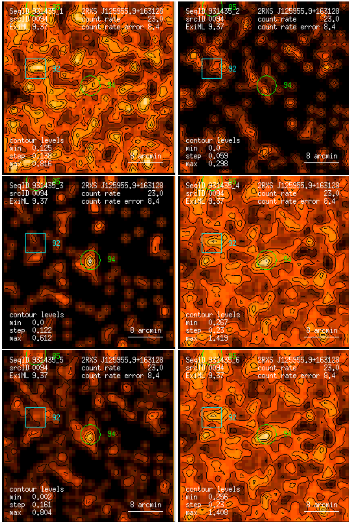
Figure 94: RASS 931435: detection 0094: band rate images, Gaussian filter: (1) PSPC channels 11 – 41, (2) 52 – 90, (3) 91 – 201, (4) 11 – 235, (5) 52 – 201, (6) 11 – 201. Broad band rates in counts/ks. Band rate contour levels in counts/ks/arcmin 2 .
