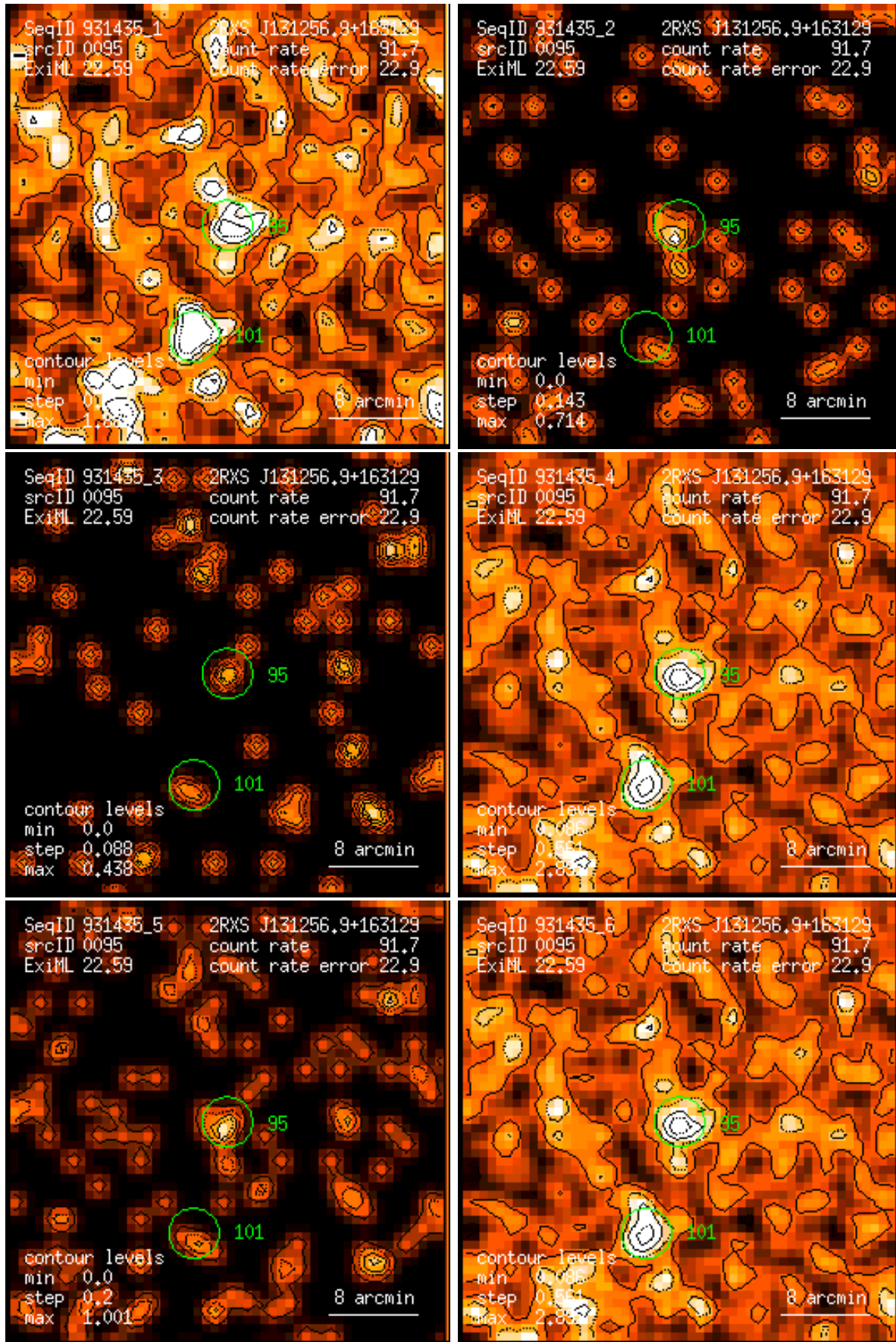
Figure 95: RASS 931435: detection 0095: band rate images, Gaussian filter: (1) PSPC channels 11 – 41, (2) 52 – 90, (3) 91 – 201, (4) 11 – 235, (5) 52 – 201, (6) 11 – 201. Broad band rates in counts/ks. Band rate contour levels in counts/ks/arcmin 2 .
