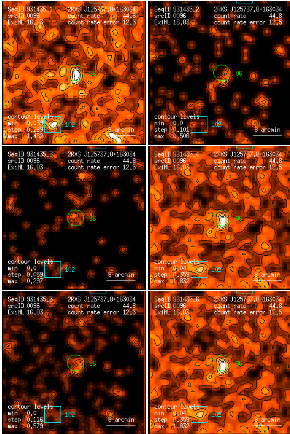
Figure 96: RASS 931435: detection 0096: band rate images, Gaussian filter: (1) PSPC channels 11 – 41, (2) 52 – 90, (3) 91 – 201, (4) 11 – 235, (5) 52 – 201, (6) 11 – 201. Broad band rates in counts/ks. Band rate contour levels in counts/ks/arcmin 2 .
