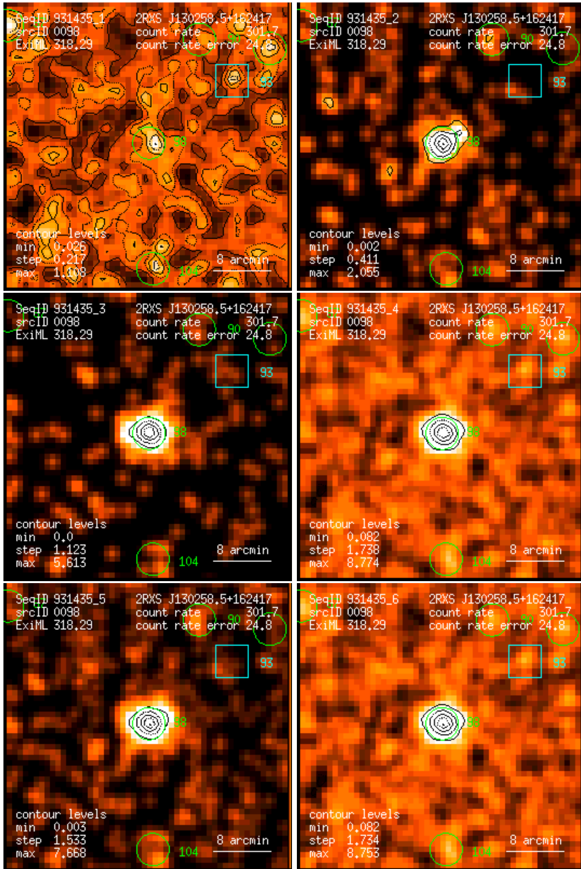
Figure 98: RASS 931435: detection 0098: band rate images, Gaussian filter: (1) PSPC channels 11 – 41, (2) 52 – 90, (3) 91 – 201, (4) 11 – 235, (5) 52 – 201, (6) 11 – 201. Broad band rates in counts/ks. Band rate contour levels in counts/ks/arcmin 2 .
