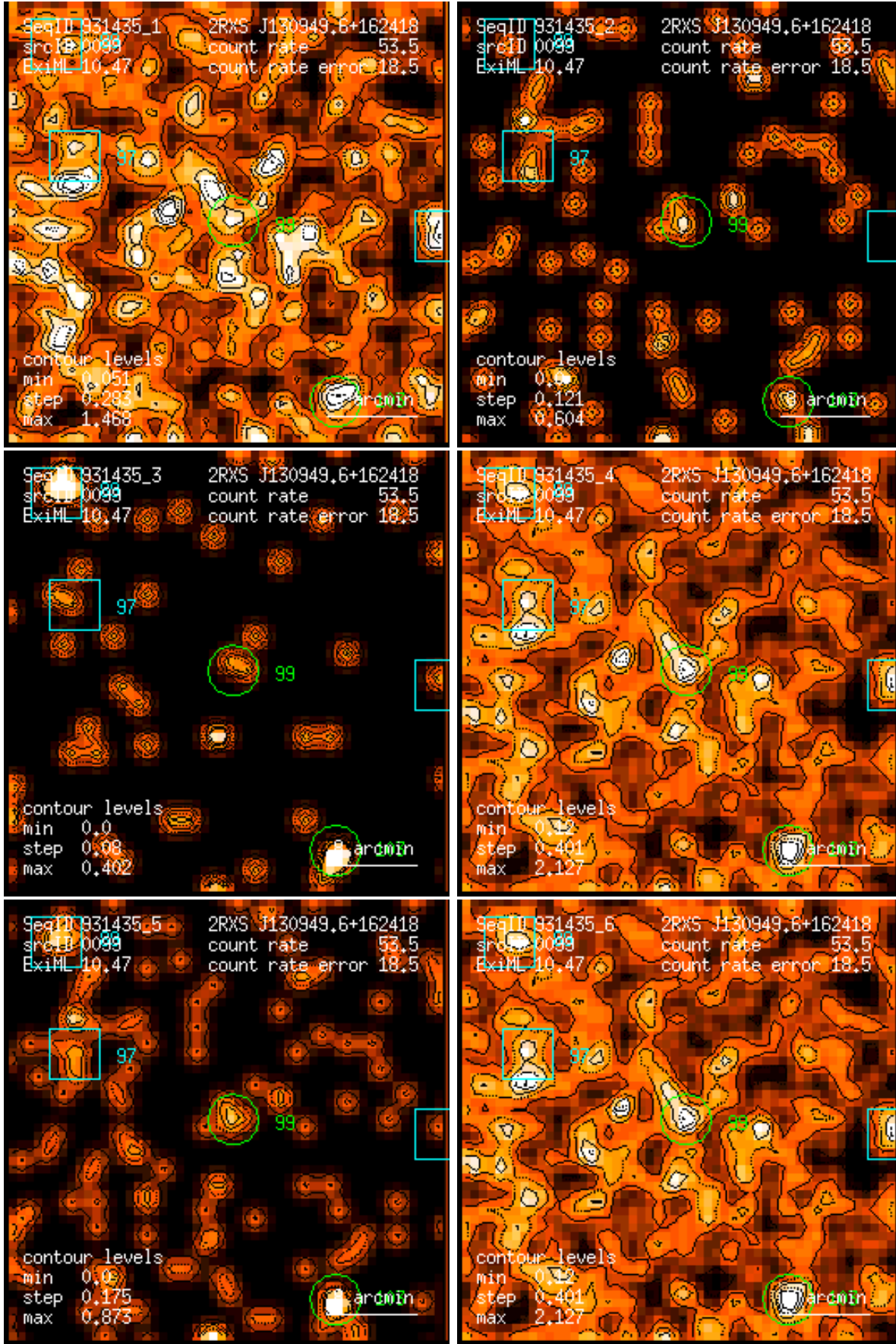
Figure 99: RASS 931435: detection 0099: band rate images, Gaussian filter: (1) PSPC channels 11 – 41, (2) 52 – 90, (3) 91 – 201, (4) 11 – 235, (5) 52 – 201, (6) 11 – 201. Broad band rates in counts/ks. Band rate contour levels in counts/ks/arcmin 2 .
