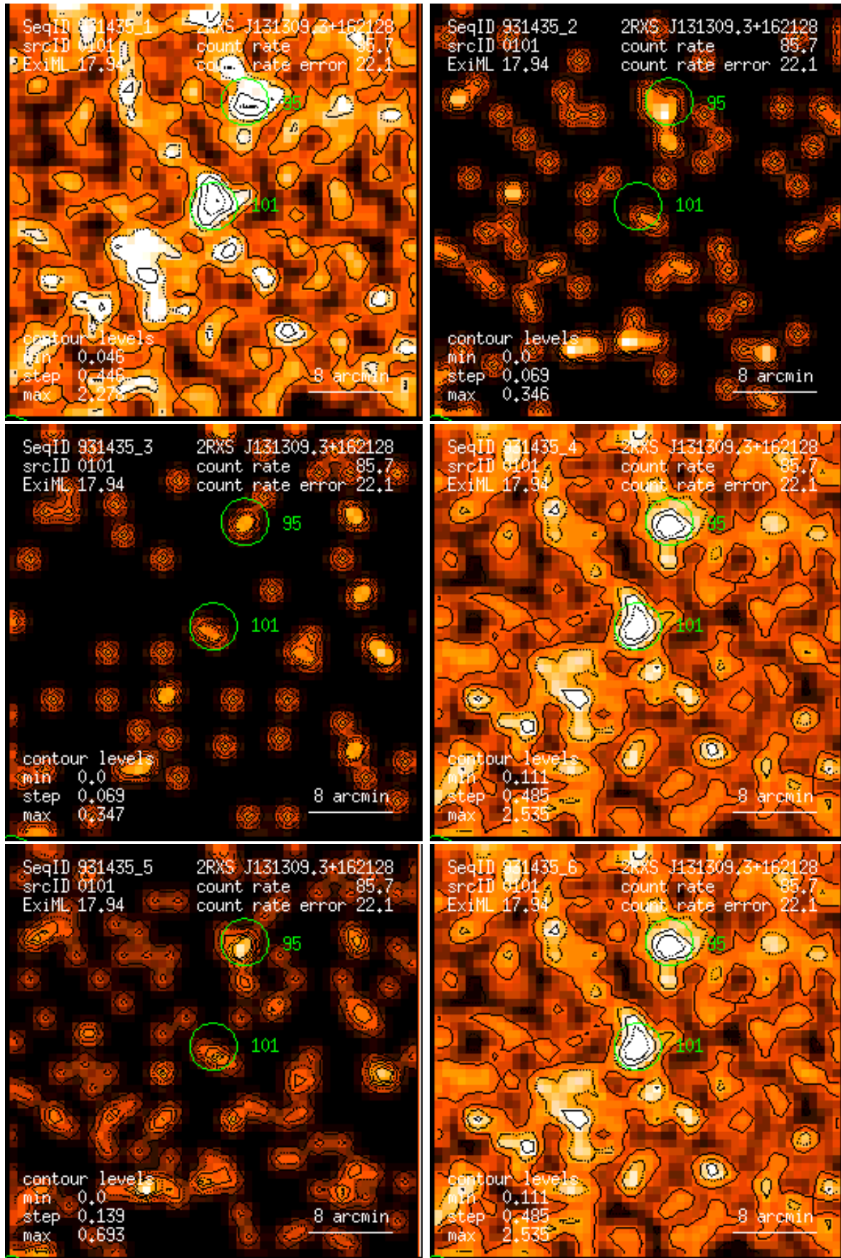
Figure 101: RASS 931435: detection 0101: band rate images, Gaussian filter: (1) PSPC channels 11 – 41, (2) 52 – 90, (3) 91 – 201, (4) 11 – 235, (5) 52 – 201, (6) 11 – 201. Broad band rates in counts/ks. Band rate contour levels in counts/ks/arcmin 2 .
