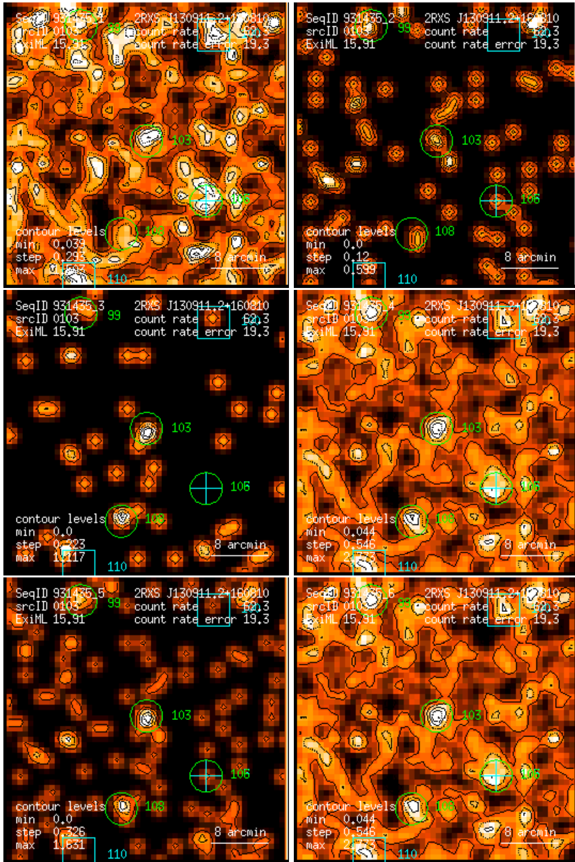
Figure 103: RASS 931435: detection 0103: band rate images, Gaussian filter: (1) PSPC channels 11 – 41, (2) 52 – 90, (3) 91 – 201, (4) 11 – 235, (5) 52 – 201, (6) 11 – 201. Broad band rates in counts/ks. Band rate contour levels in counts/ks/arcmin 2 .
