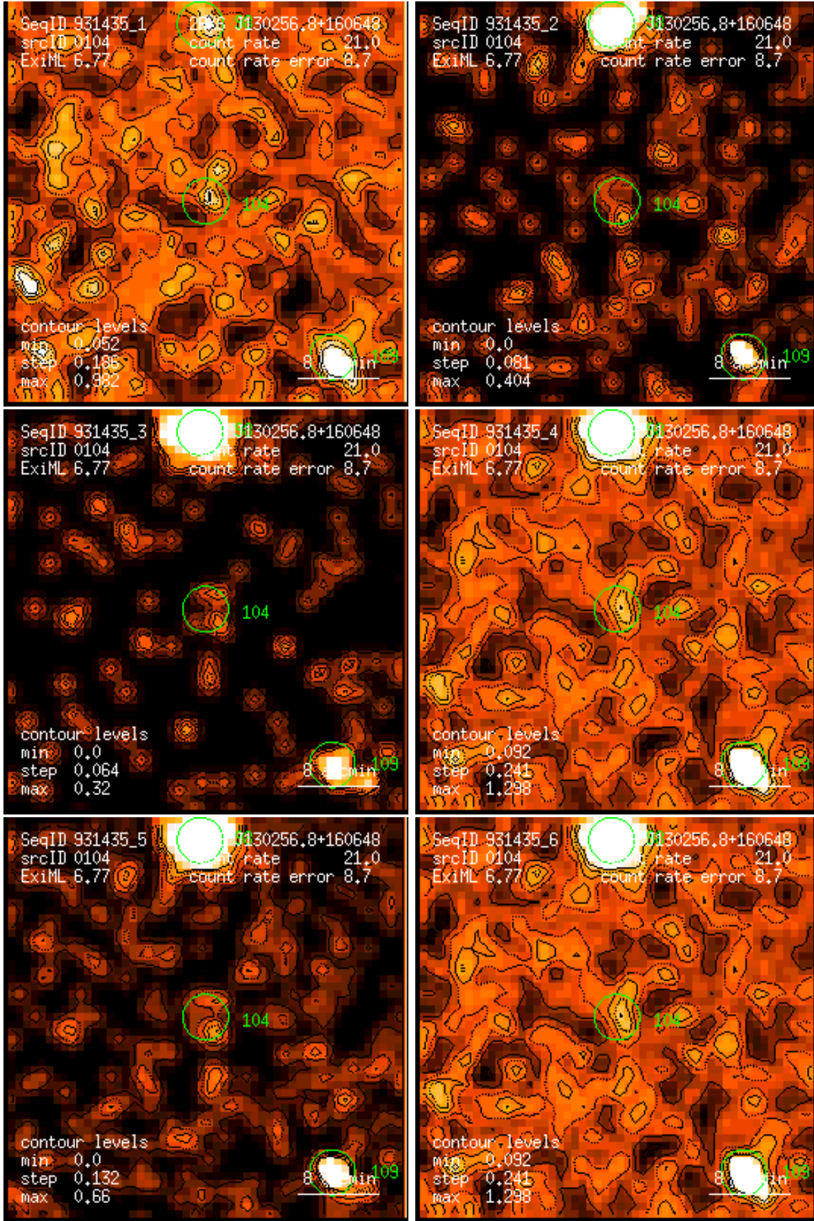
Figure 104: RASS 931435: detection 0104: band rate images, Gaussian filter: (1) PSPC channels 11 – 41, (2) 52 – 90, (3) 91 – 201, (4) 11 – 235, (5) 52 – 201, (6) 11 – 201. Broad band rates in counts/ks. Band rate contour levels in counts/ks/arcmin 2 .
