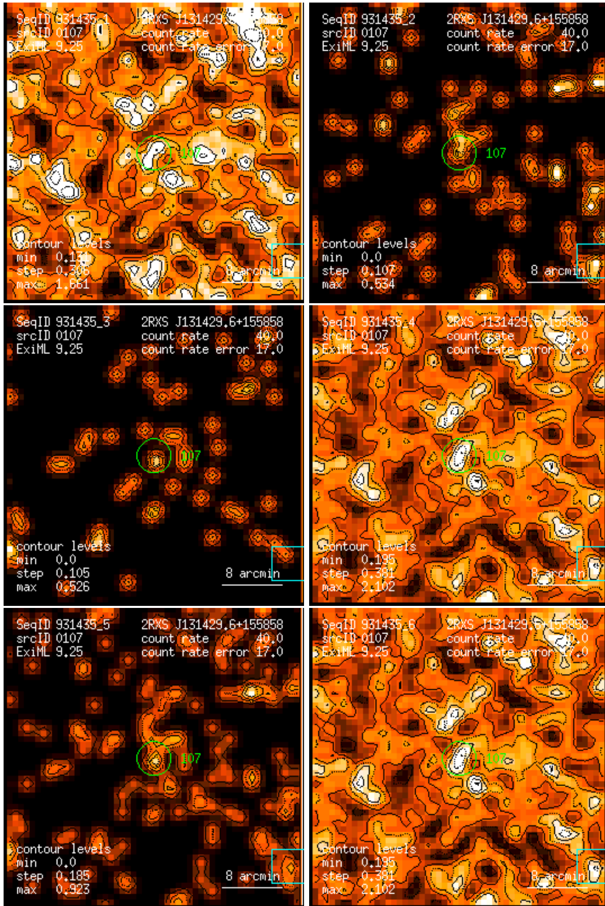
Figure 107: RASS 931435: detection 0107: band rate images, Gaussian filter: (1) PSPC channels 11 – 41, (2) 52 – 90, (3) 91 – 201, (4) 11 – 235, (5) 52 – 201, (6) 11 – 201. Broad band rates in counts/ks. Band rate contour levels in counts/ks/arcmin 2 .
