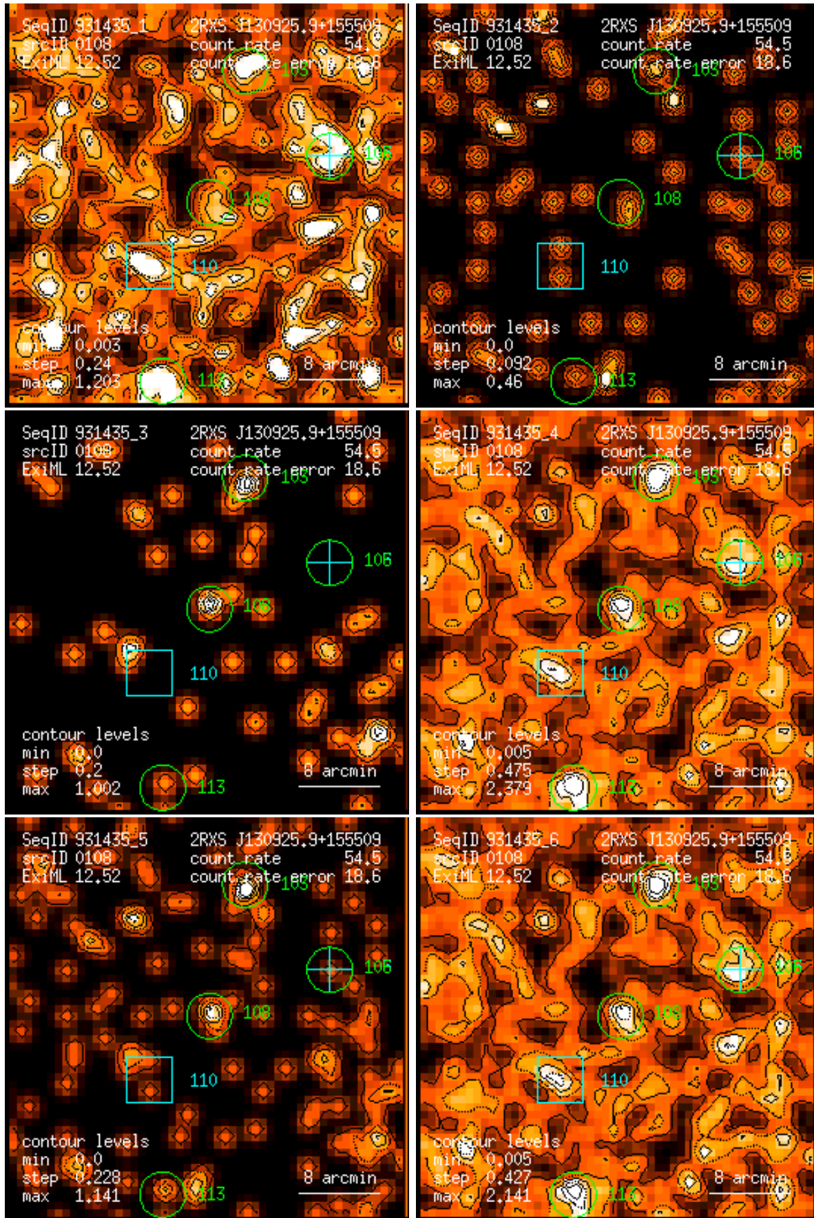
Figure 108: RASS 931435: detection 0108: band rate images, Gaussian filter: (1) PSPC channels 11 – 41, (2) 52 – 90, (3) 91 – 201, (4) 11 – 235, (5) 52 – 201, (6) 11 – 201. Broad band rates in counts/ks. Band rate contour levels in counts/ks/arcmin 2 .
