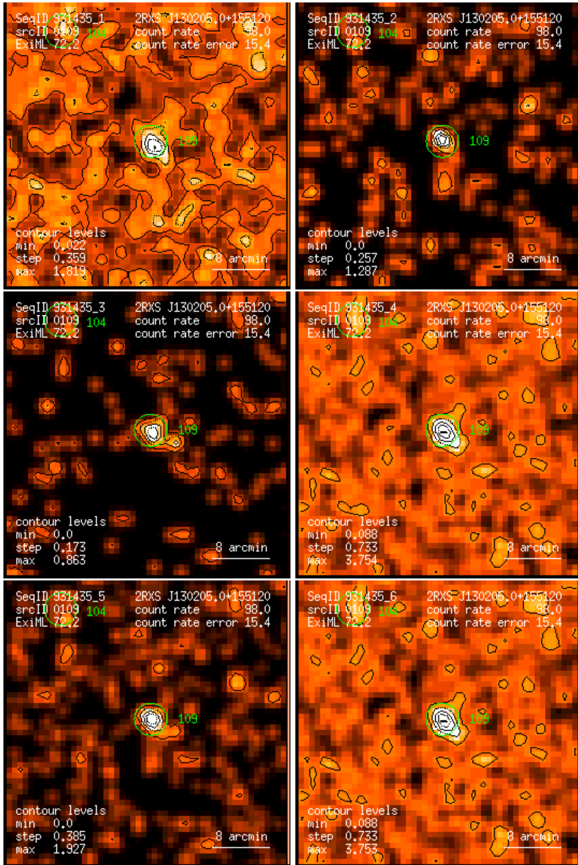
Figure 109: RASS 931435: detection 0109: band rate images, Gaussian filter: (1) PSPC channels 11 – 41, (2) 52 – 90, (3) 91 – 201, (4) 11 – 235, (5) 52 – 201, (6) 11 – 201. Broad band rates in counts/ks. Band rate contour levels in counts/ks/arcmin 2 .
