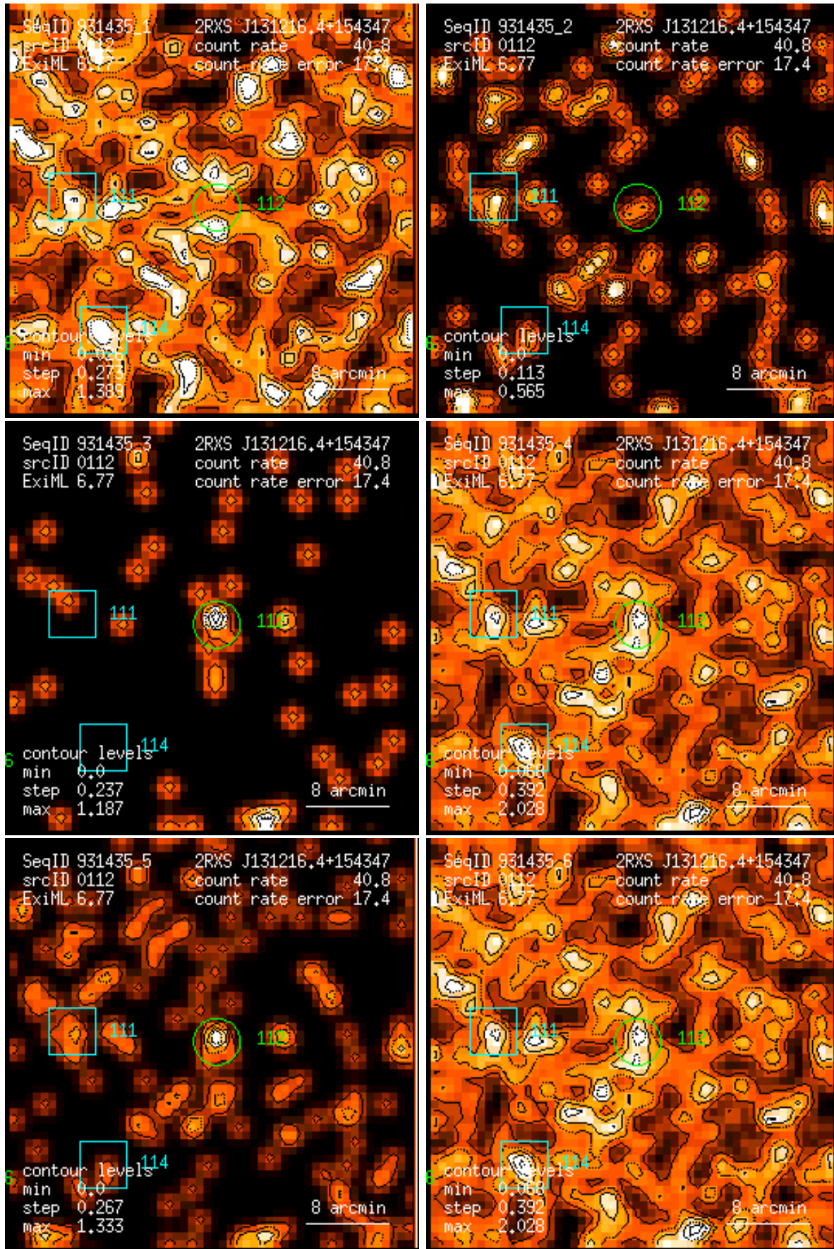
Figure 112: RASS 931435: detection 0112: band rate images, Gaussian filter: (1) PSPC channels 11 – 41, (2) 52 – 90, (3) 91 – 201, (4) 11 – 235, (5) 52 – 201, (6) 11 – 201. Broad band rates in counts/ks. Band rate contour levels in counts/ks/arcmin 2 .
