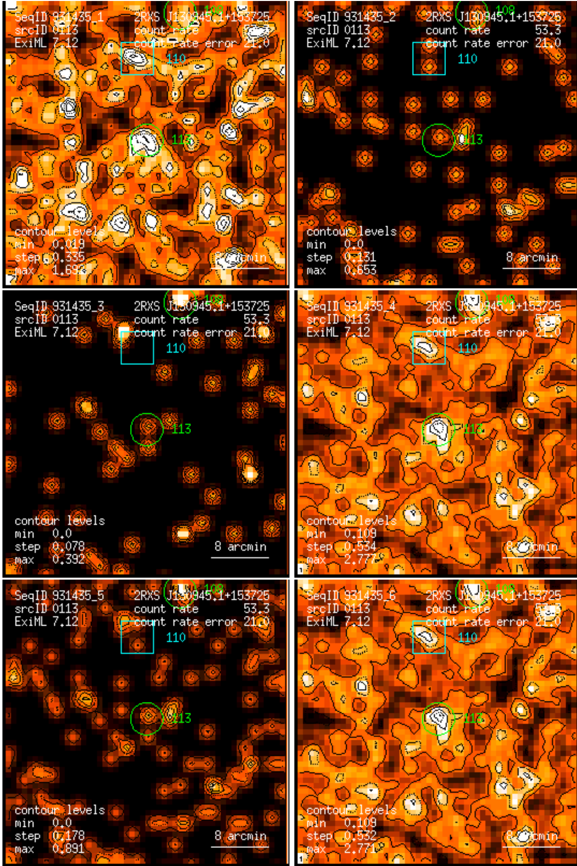
Figure 113: RASS 931435: detection 0113: band rate images, Gaussian filter: (1) PSPC channels 11 – 41, (2) 52 – 90, (3) 91 – 201, (4) 11 – 235, (5) 52 – 201, (6) 11 – 201. Broad band rates in counts/ks. Band rate contour levels in counts/ks/arcmin 2 .
