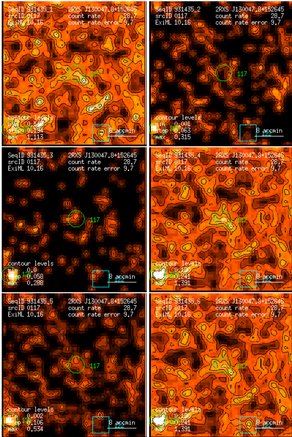
Figure 117: RASS 931435: detection 0117: band rate images, Gaussian filter: (1) PSPC channels 11 – 41, (2) 52 – 90, (3) 91 – 201, (4) 11 – 235, (5) 52 – 201, (6) 11 – 201. Broad band rates in counts/ks. Band rate contour levels in counts/ks/arcmin 2 .
