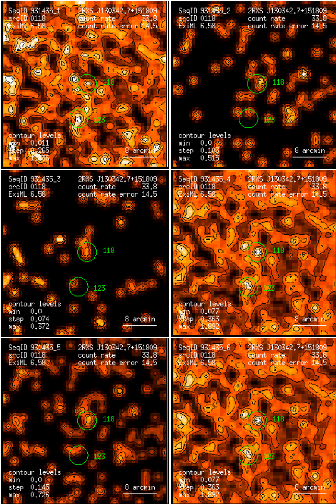
Figure 118: RASS 931435: detection 0118: band rate images, Gaussian filter: (1) PSPC channels 11 – 41, (2) 52 – 90, (3) 91 – 201, (4) 11 – 235, (5) 52 – 201, (6) 11 – 201. Broad band rates in counts/ks. Band rate contour levels in counts/ks/arcmin 2 .
