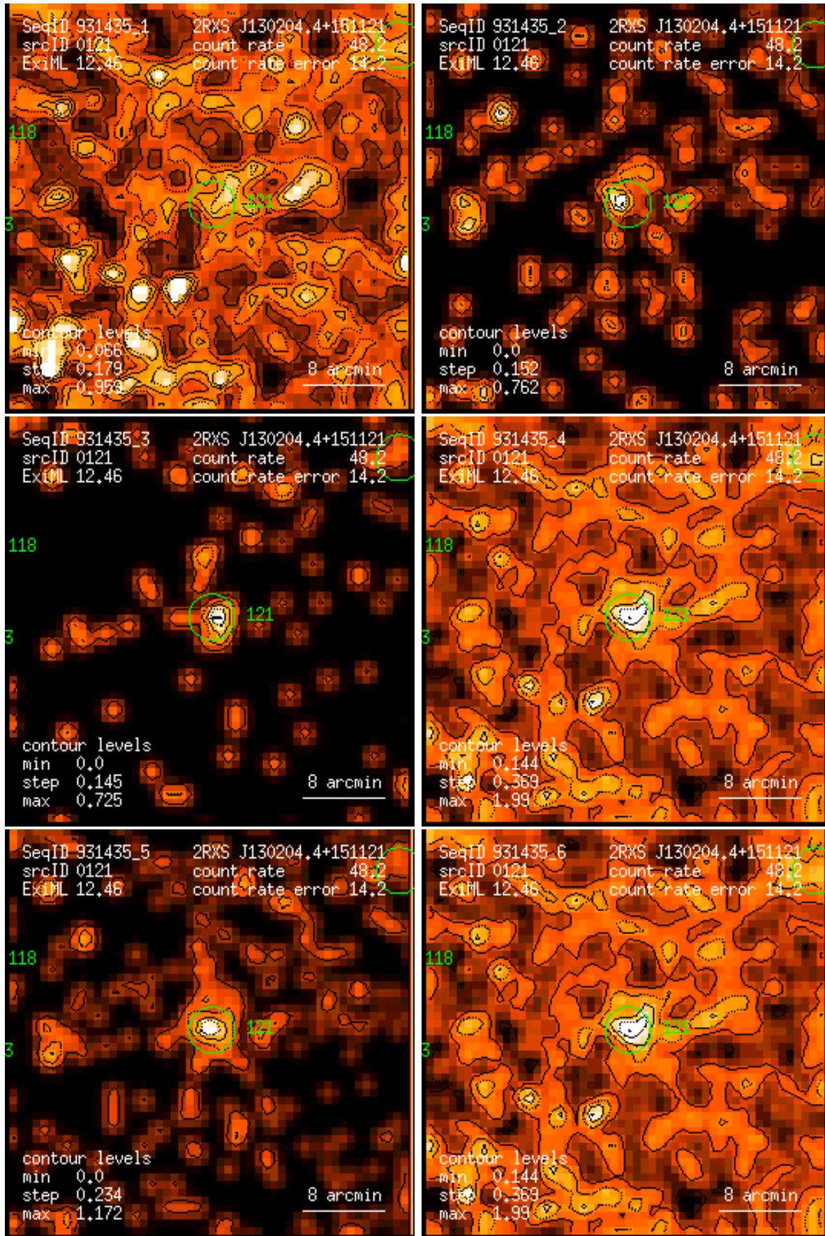
Figure 121: RASS 931435: detection 0121: band rate images, Gaussian filter: (1) PSPC channels 11 – 41, (2) 52 – 90, (3) 91 – 201, (4) 11 – 235, (5) 52 – 201, (6) 11 – 201. Broad band rates in counts/ks. Band rate contour levels in counts/ks/arcmin 2 .
