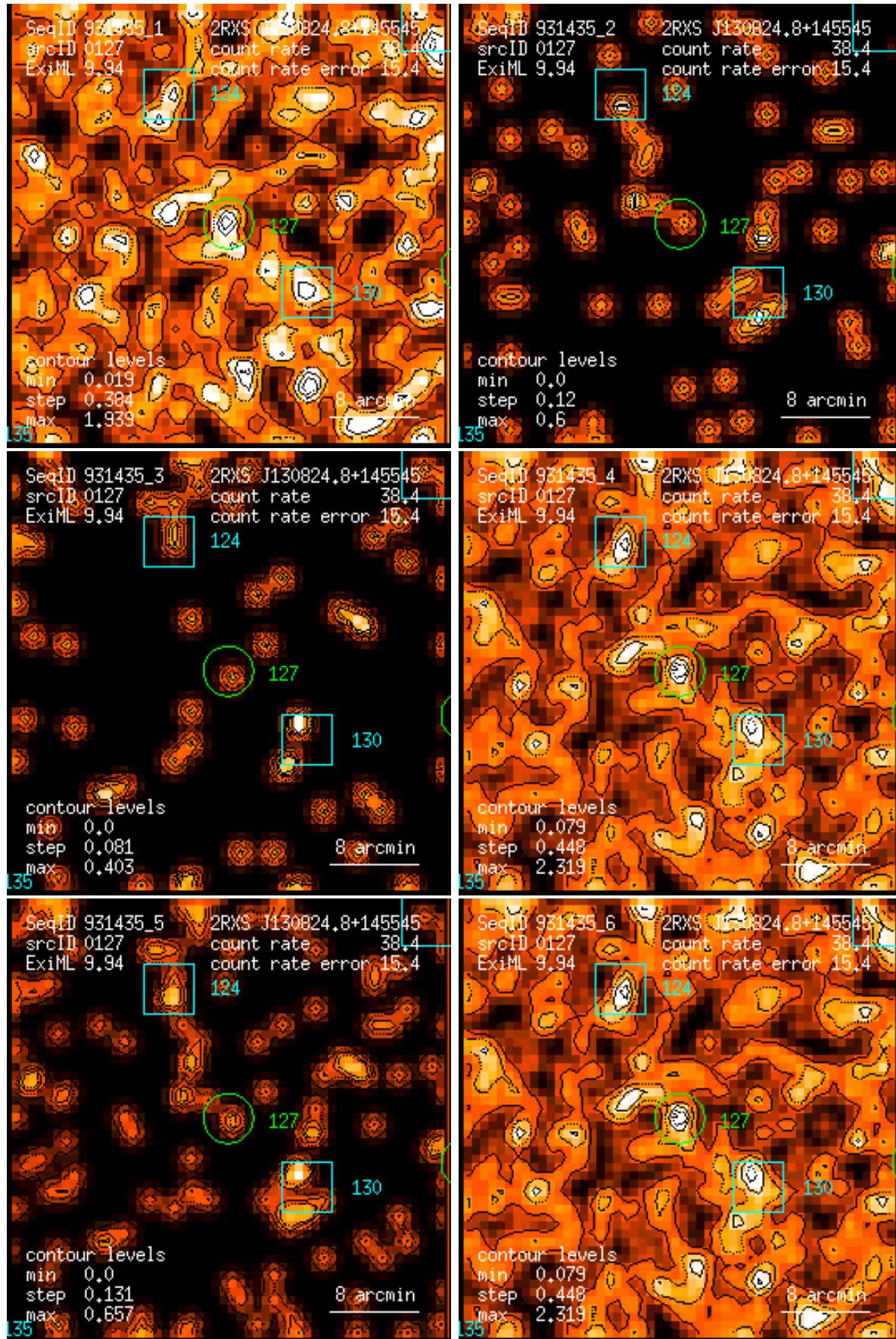
Figure 127: RASS 931435: detection 0127: band rate images, Gaussian filter: (1) PSPC channels 11 – 41, (2) 52 – 90, (3) 91 – 201, (4) 11 – 235, (5) 52 – 201, (6) 11 – 201. Broad band rates in counts/ks. Band rate contour levels in counts/ks/arcmin 2 .
