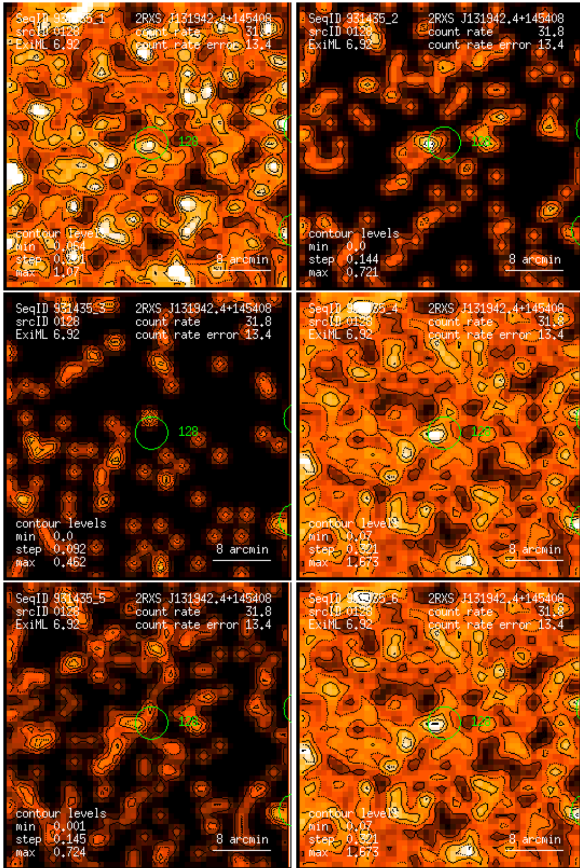
Figure 128: RASS 931435: detection 0128: band rate images, Gaussian filter: (1) PSPC channels 11 – 41, (2) 52 – 90, (3) 91 – 201, (4) 11 – 235, (5) 52 – 201, (6) 11 – 201. Broad band rates in counts/ks. Band rate contour levels in counts/ks/arcmin 2 .
