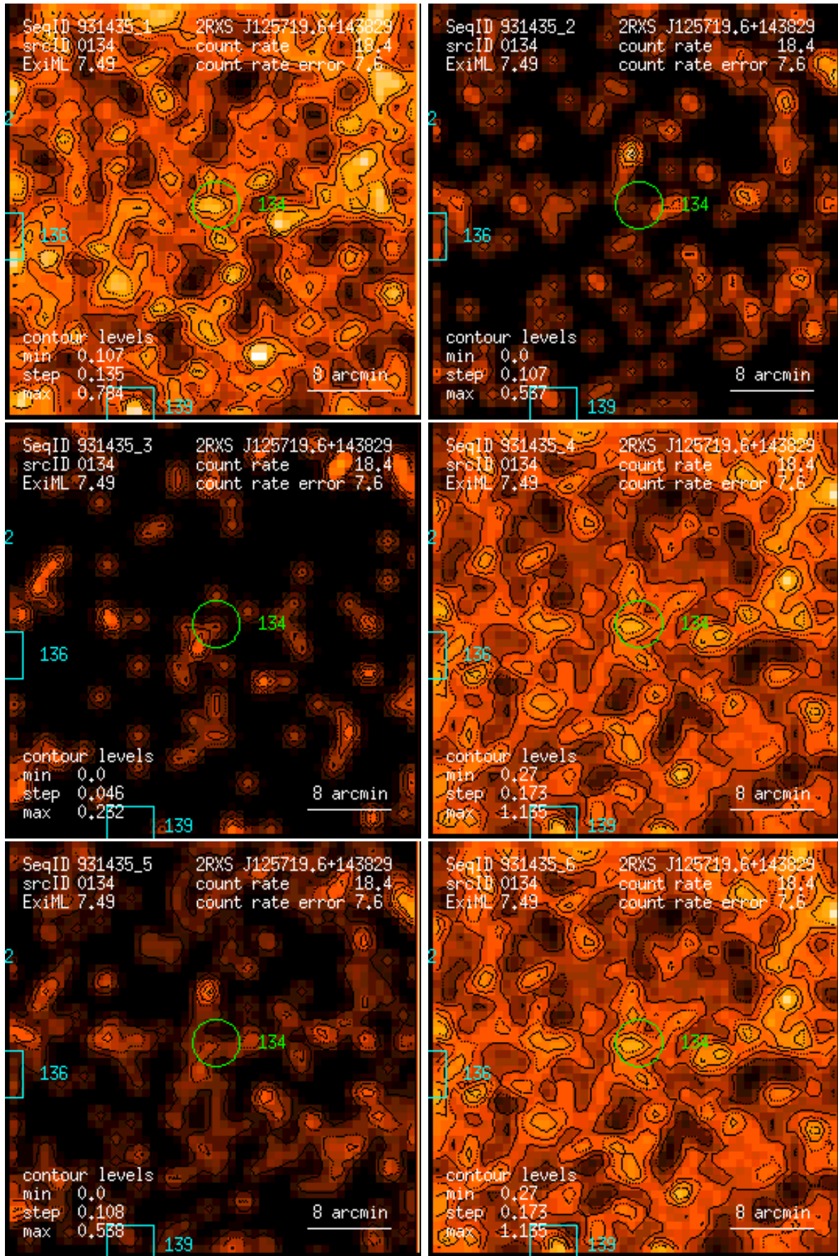
Figure 134: RASS 931435: detection 0134: band rate images, Gaussian filter: (1) PSPC channels 11 – 41, (2) 52 – 90, (3) 91 – 201, (4) 11 – 235, (5) 52 – 201, (6) 11 – 201. Broad band rates in counts/ks. Band rate contour levels in counts/ks/arcmin 2 .
