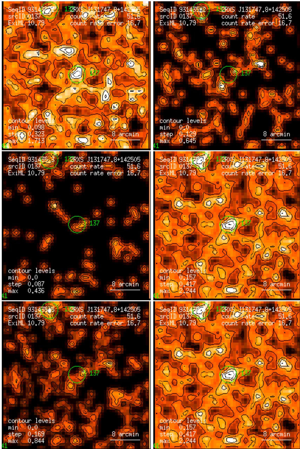
Figure 137: RASS 931435: detection 0137: band rate images, Gaussian filter: (1) PSPC channels 11 – 41, (2) 52 – 90, (3) 91 – 201, (4) 11 – 235, (5) 52 – 201, (6) 11 – 201. Broad band rates in counts/ks. Band rate contour levels in counts/ks/arcmin 2 .
