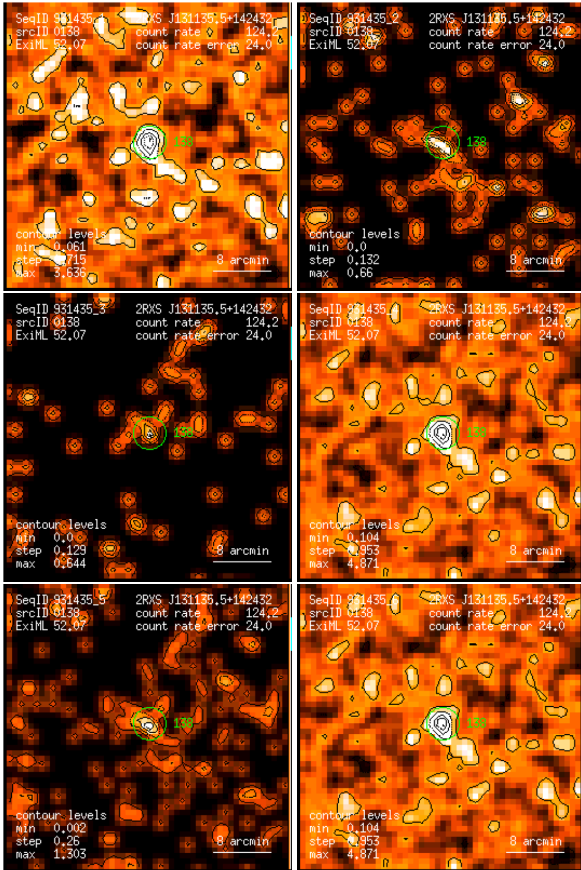
Figure 138: RASS 931435: detection 0138: band rate images, Gaussian filter: (1) PSPC channels 11 – 41, (2) 52 – 90, (3) 91 – 201, (4) 11 – 235, (5) 52 – 201, (6) 11 – 201. Broad band rates in counts/ks. Band rate contour levels in counts/ks/arcmin 2 .
